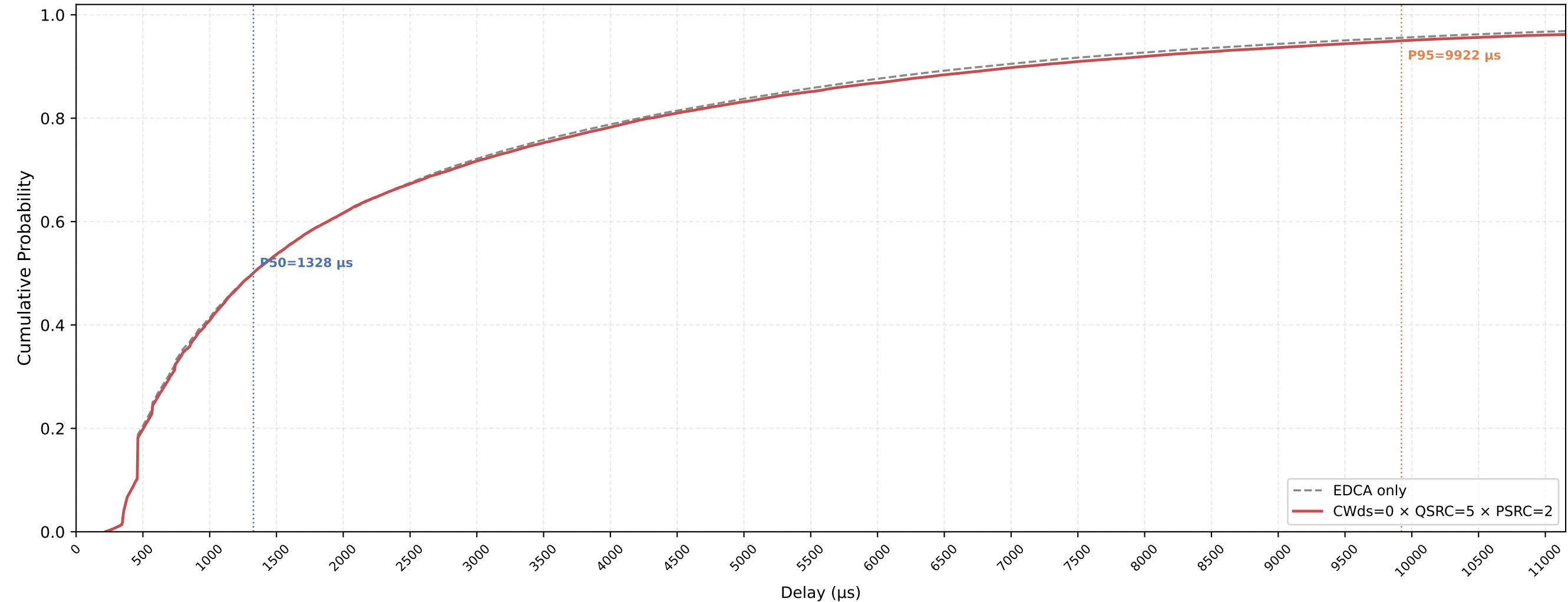
P-EDCA STA VO Delay CDF — CWds=0 × QSRC=5 × PSRC=2 nSta=30, nPedca=5, 1Mbps, avg of 10 runs
