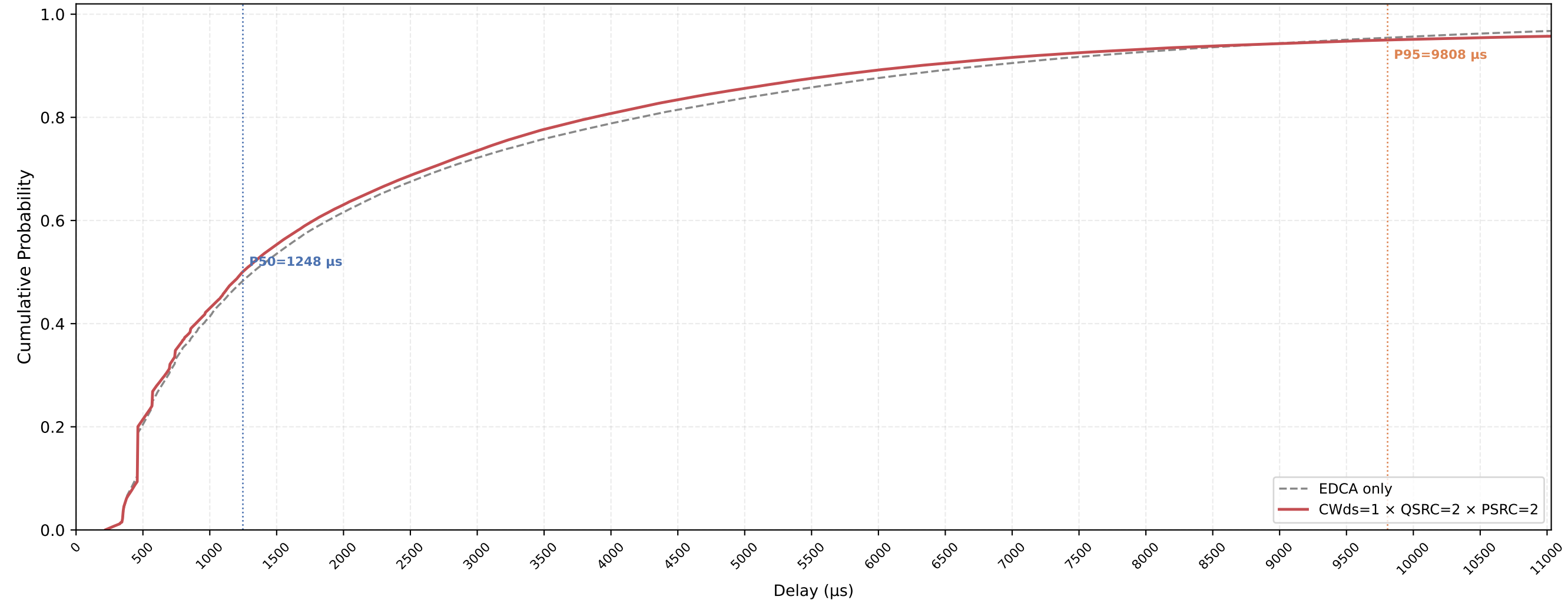
P-EDCA STA VO Delay CDF — CWds=1 × QSRC=2 × PSRC=2 nSta=30, nPedca=30, 1Mbps, avg of 10 runs
