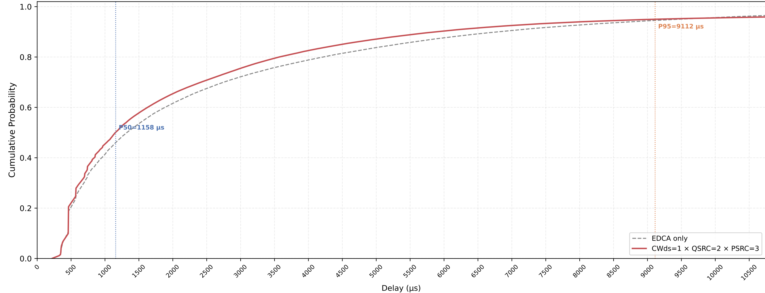
P-EDCA STA VO Delay CDF — CWds=1 × QSRC=2 × PSRC=3 nSta=30, nPedca=30, 1Mbps, avg of 10 runs
