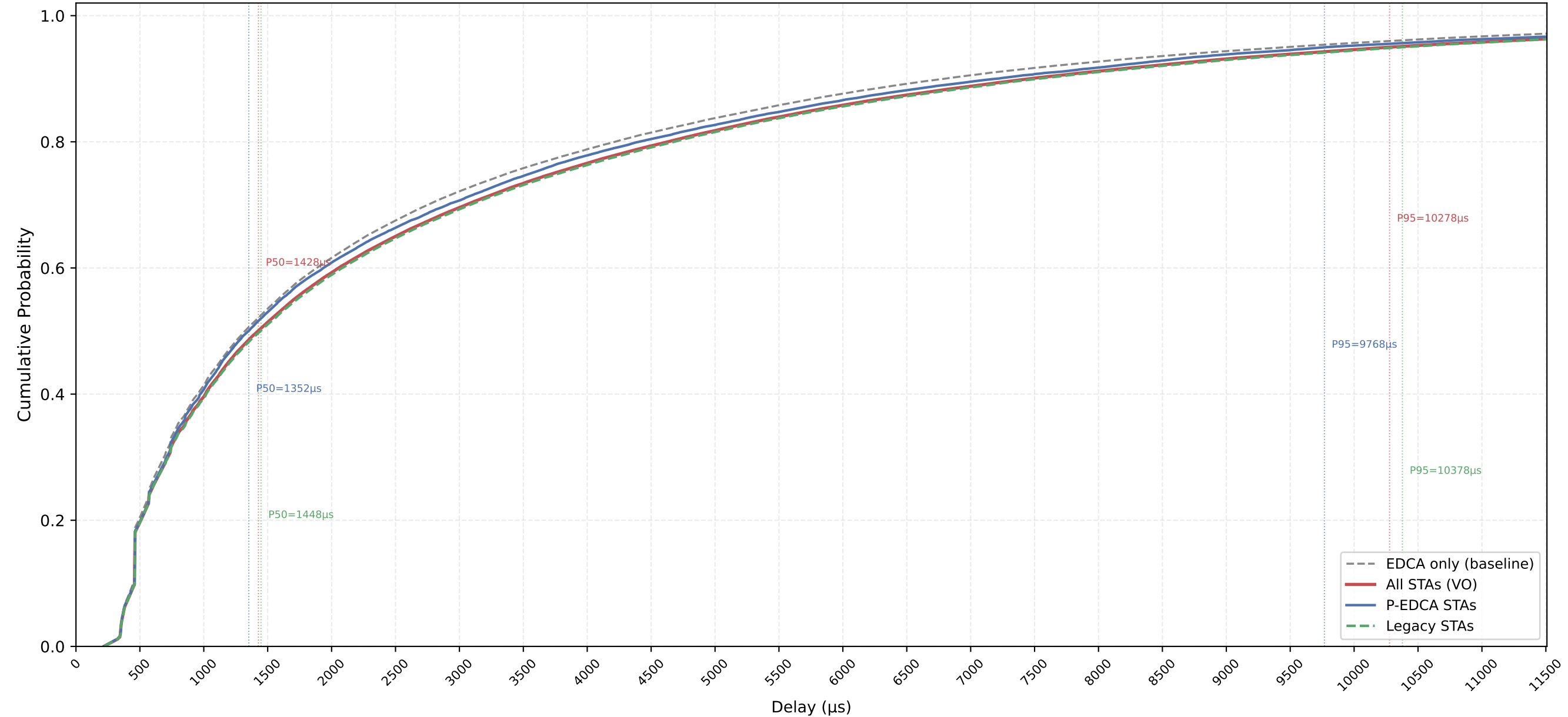
VO Delay CDF — P-EDCA / Legacy / All | CWds=1 × QSRC=4 × PSRC=2 nSta=30, nPedca=5/30, 1Mbps, avg of 10 runs
