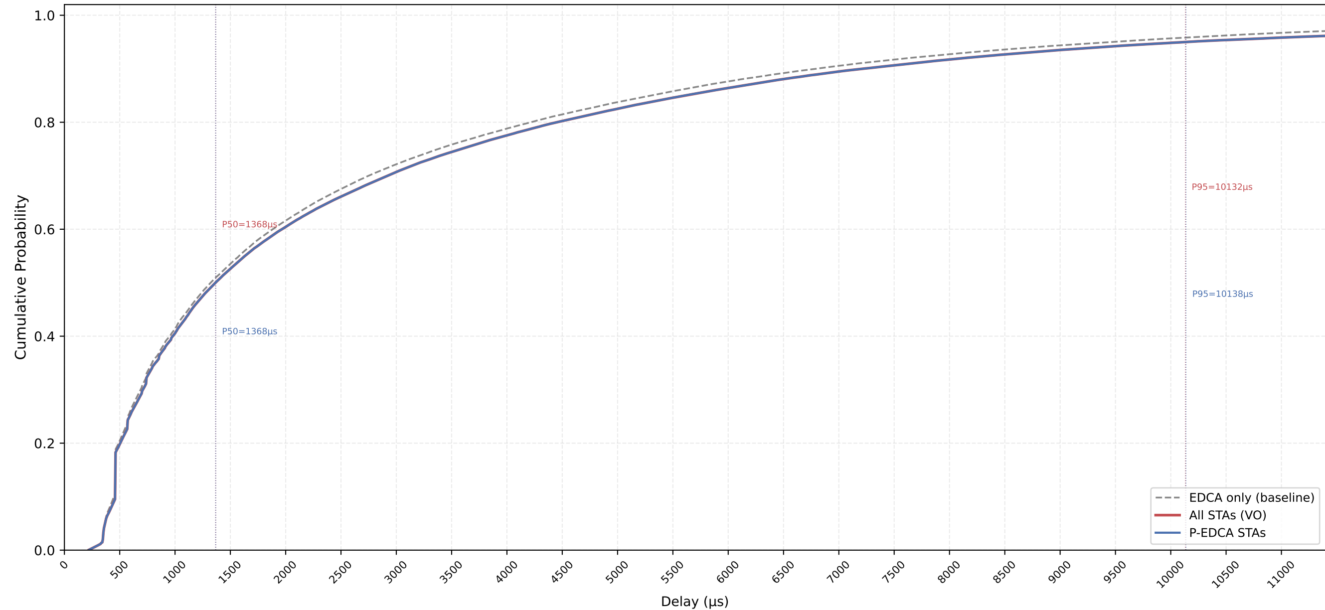
VO Delay CDF — P-EDCA / Legacy / All | CWds=1 × QSRC=4 × PSRC=2 nSta=30, nPedca=30/30, 1Mbps, avg of 10 runs
