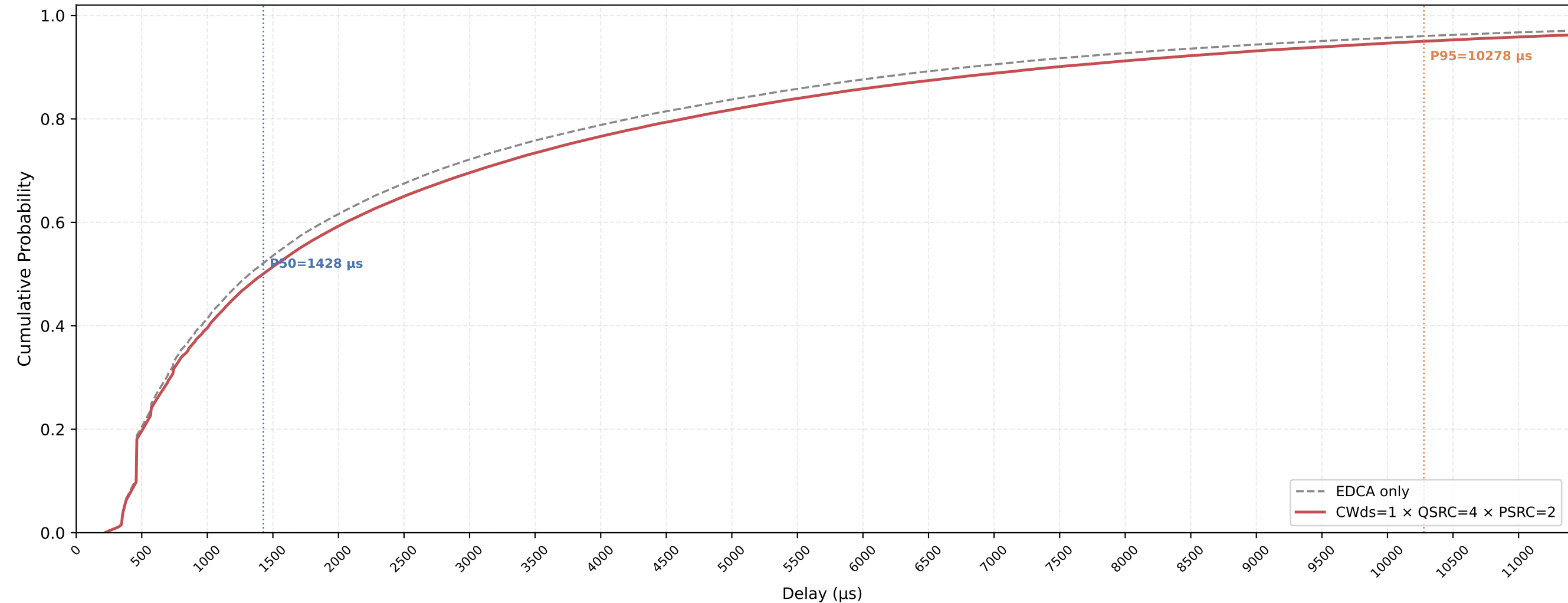
VO (all STAs) Delay CDF — CWds=1 × QSRC=4 × PSRC=2 nSta=30, nPedca=5, 1Mbps, avg of 10 runs
