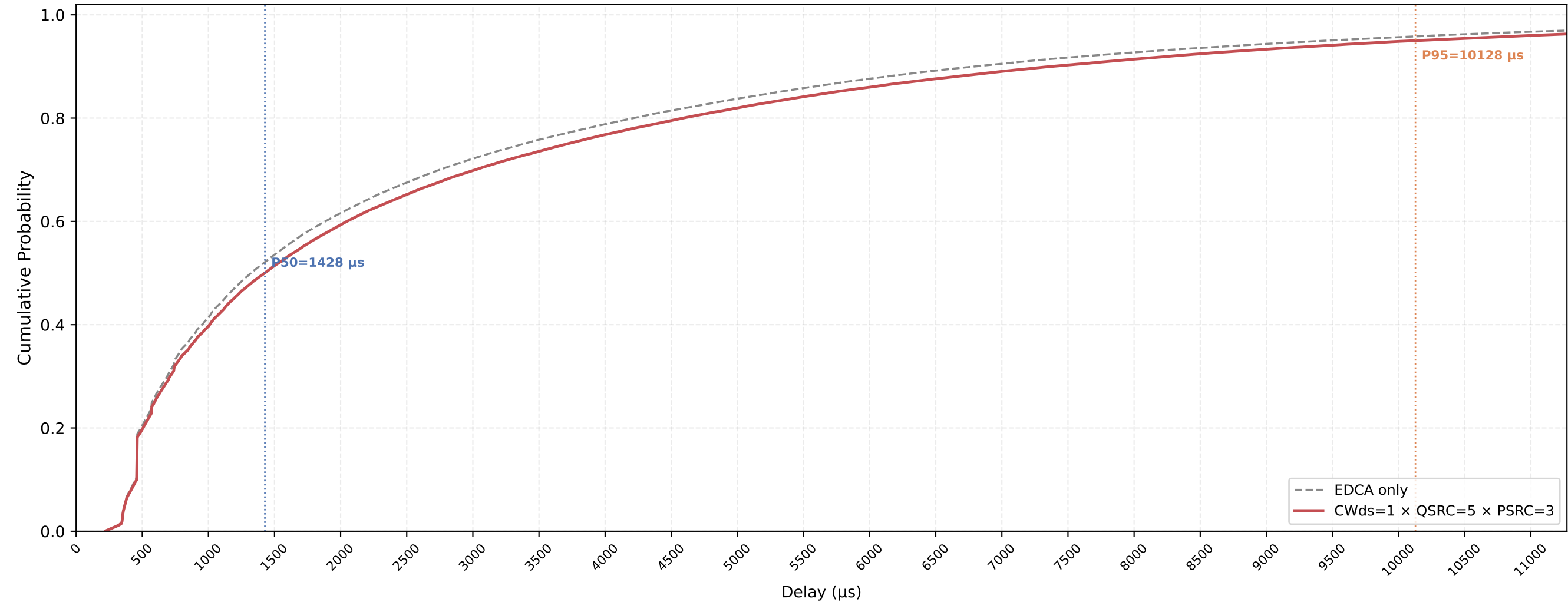
Legacy STA VO Delay CDF — CWds=1 × QSRC=5 × PSRC=3 nSta=30, nPedca=5, 1Mbps, avg of 10 runs
