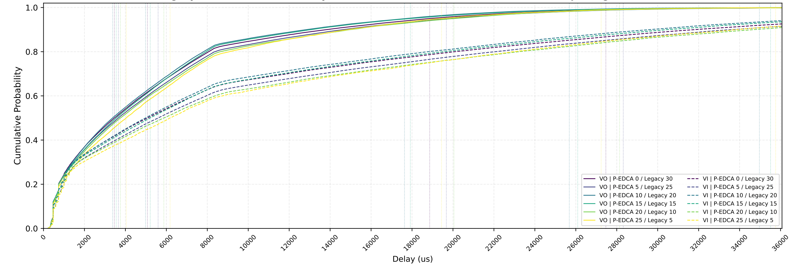
Legacy EDCA STAs VO+VI Delay CDF (VO=solid, VI=dashed) - nSta=30, 1Mbps, avg of 10 runs
