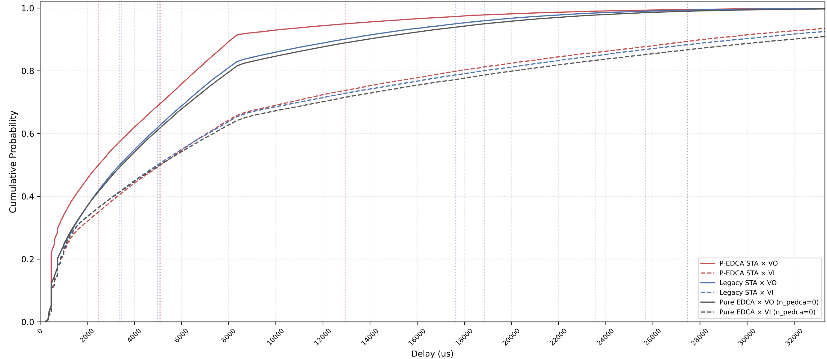
P-EDCA vs Legacy × VO/VI Delay CDF - n_pedca=10, n_legacy=20, nSta=30, 1Mbps, avg of 10 runs
