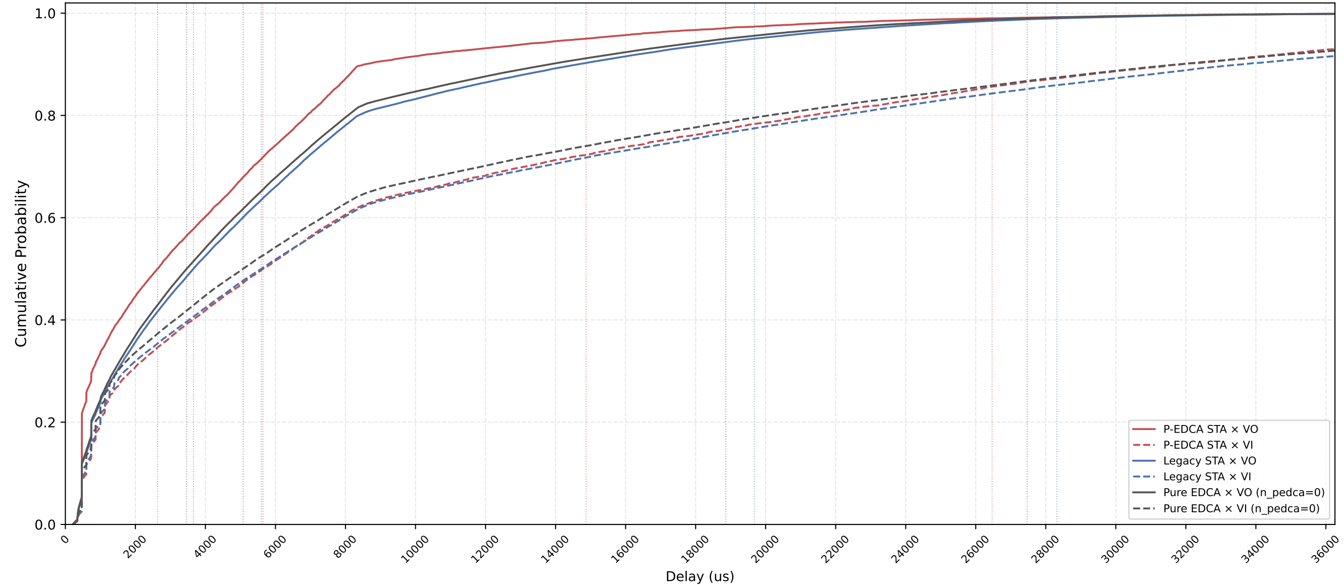
P-EDCA vs Legacy × VO/VI Delay CDF - n_pedca=5, n_legacy=25, nSta=30, 1Mbps, avg of 10 runs
