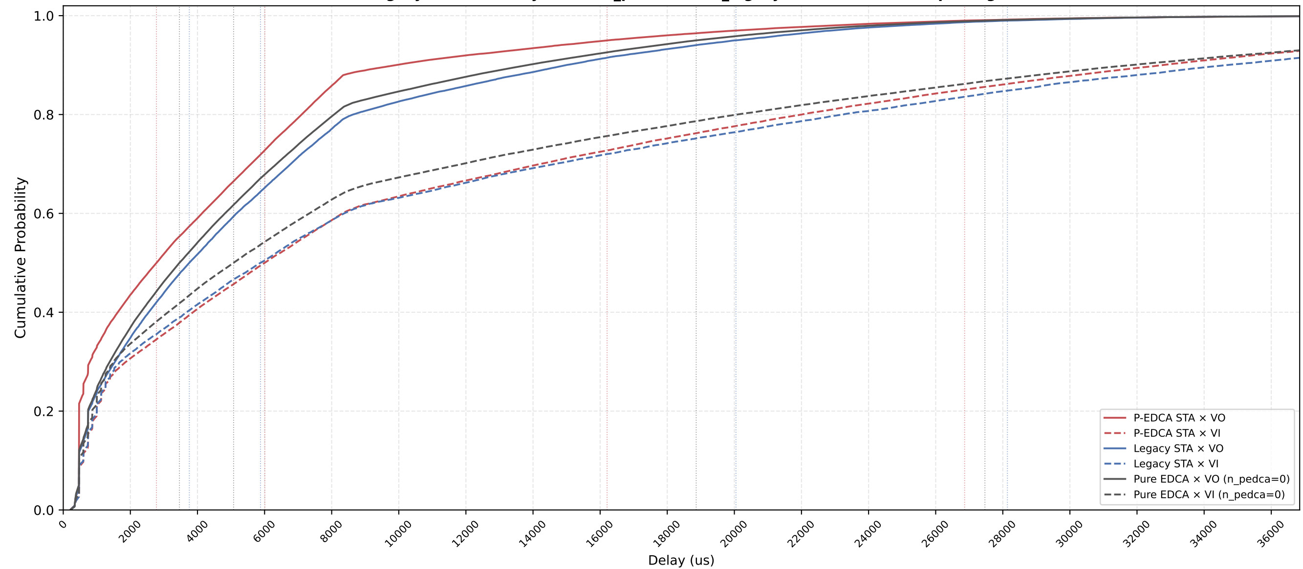
P-EDCA vs Legacy × VO/VI Delay CDF - n_pedca=20, n_legacy=10, nSta=30, 1Mbps, avg of 10 runs
