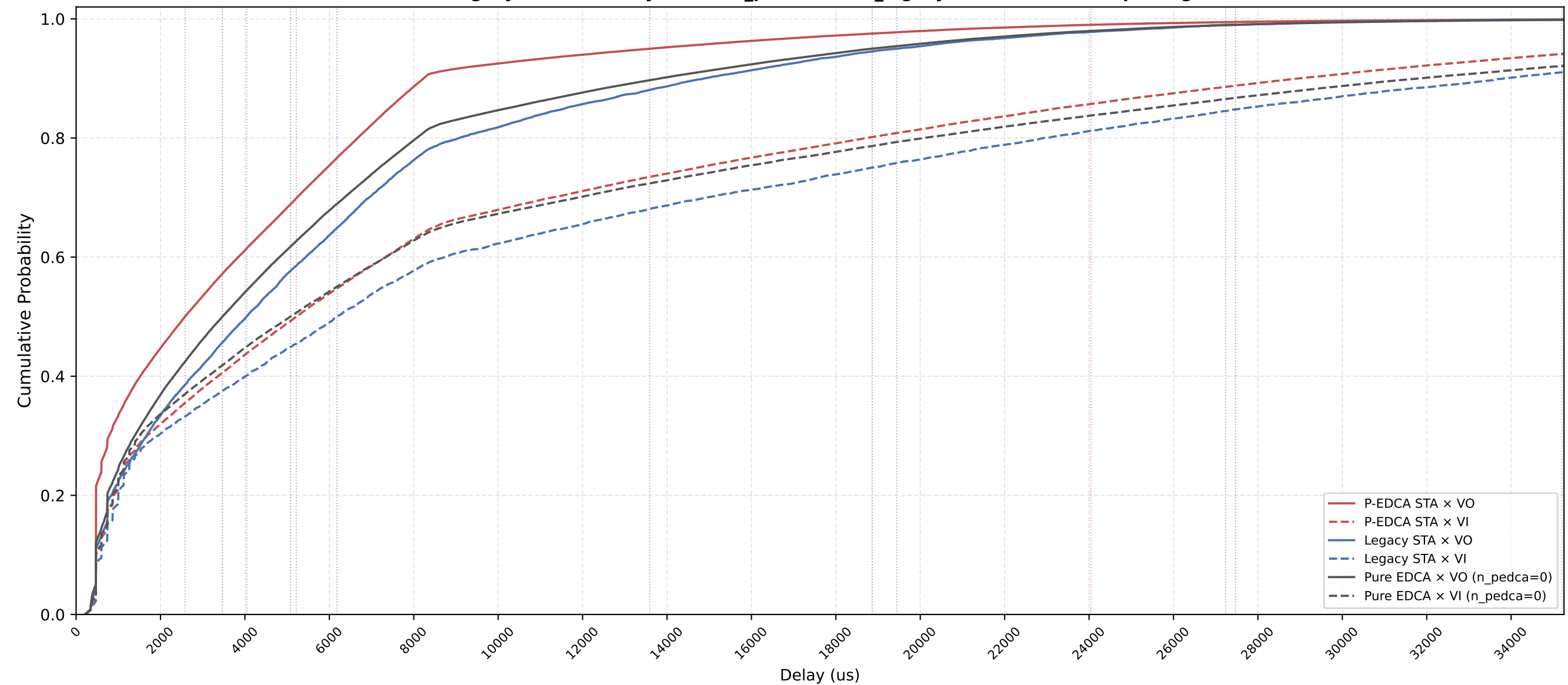
P-EDCA vs Legacy × VO/VI Delay CDF - n_pedca=25, n_legacy=5, nSta=30, 1Mbps, avg of 10 runs
