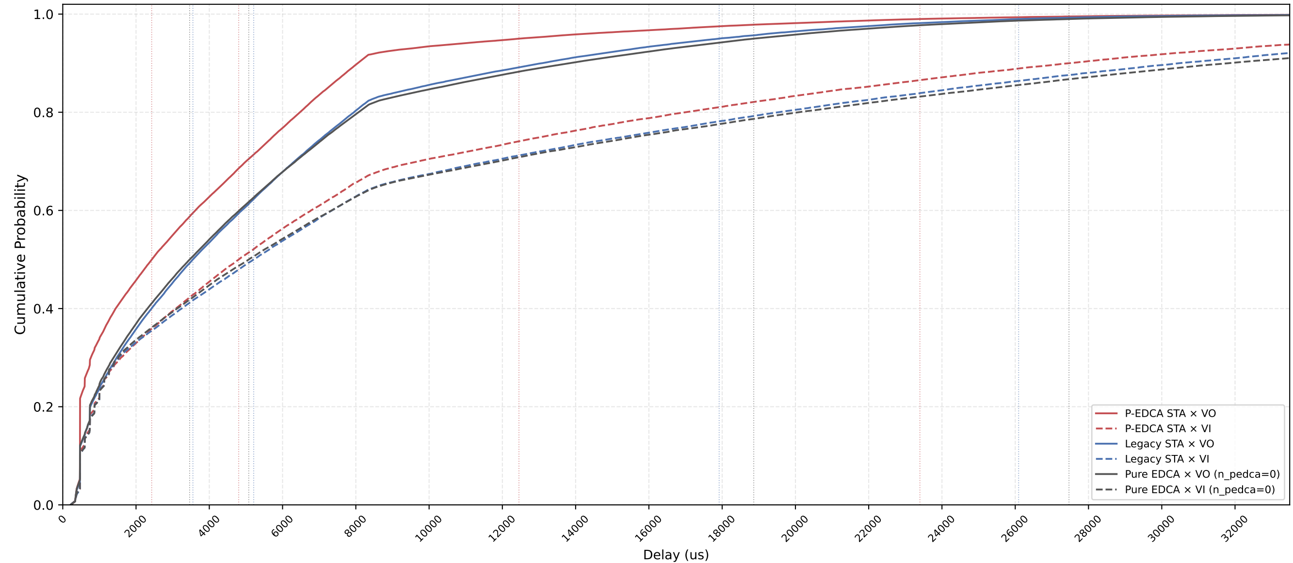
P-EDCA vs Legacy × VO/VI Delay CDF - n_pedca=15, n_legacy=15, nSta=30, 1Mbps, avg of 10 runs
