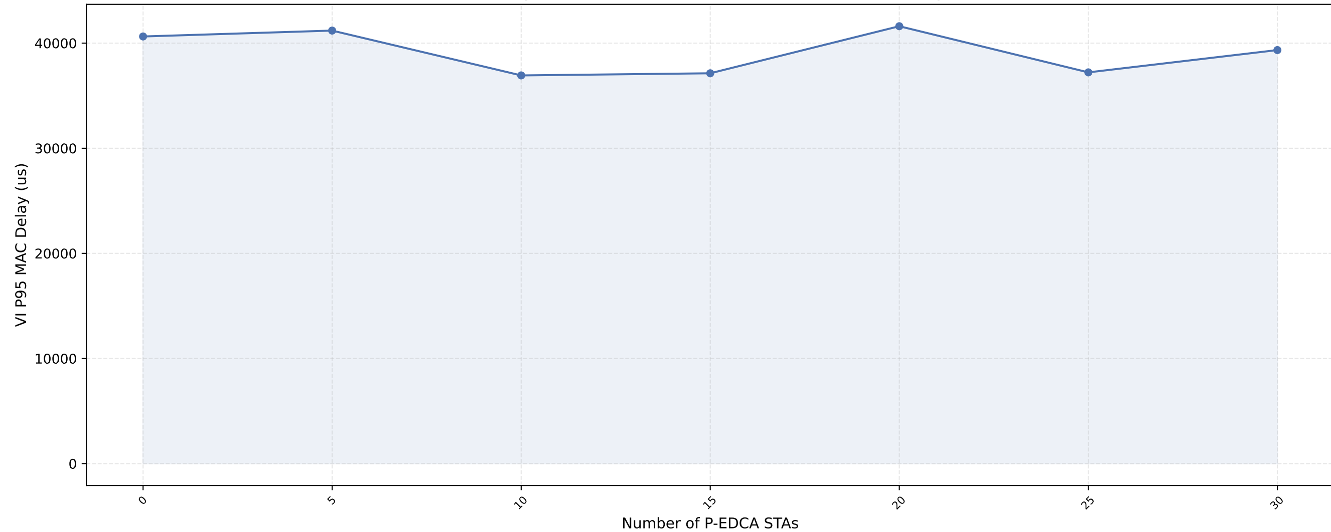
VI P95 MAC Delay vs P-EDCA STAs — nSta=30, 1Mbps (avg of 10 runs)
