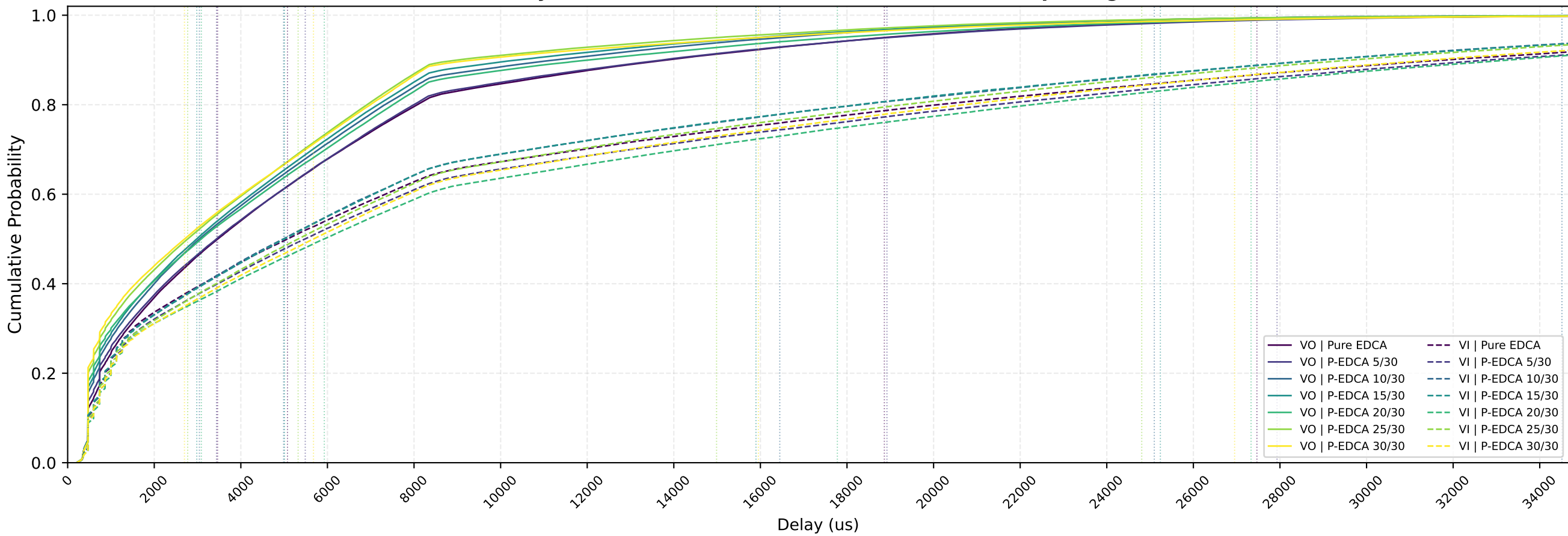
VO + VI Delay CDF (VO=solid, VI=dashed) - nSta=30, 1Mbps, avg of 10 runs
