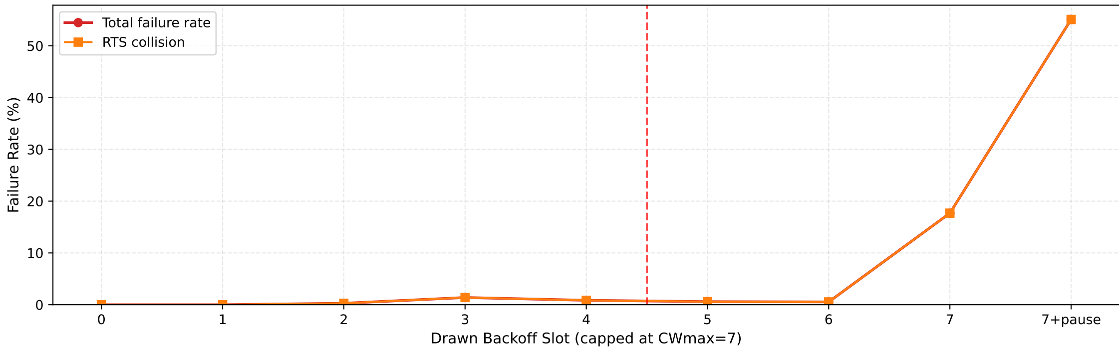
Failure Rate vs Drawn Backoff Slot
