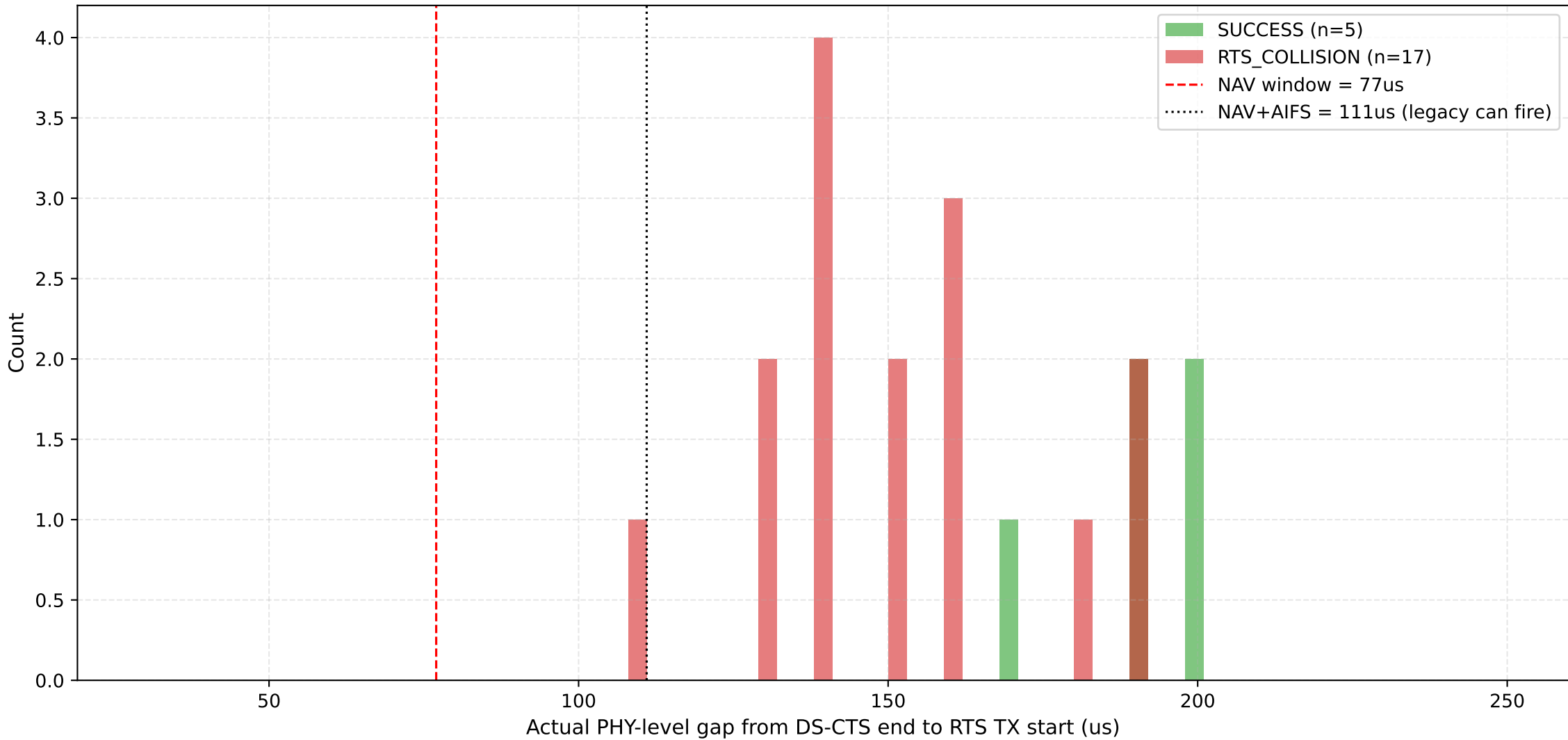
Actual RTS TX time distribution: SUCCESS vs RTS_COLLISION
