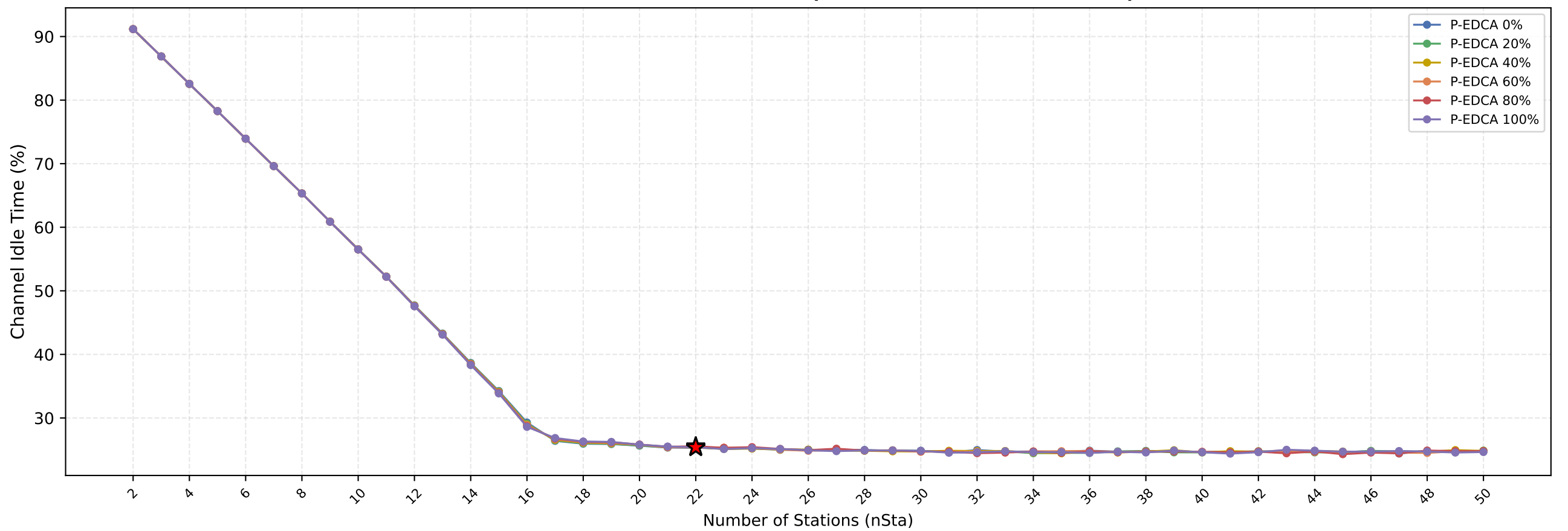
Channel Idle Time vs nSta — (Red Star = Current nSta=22)
