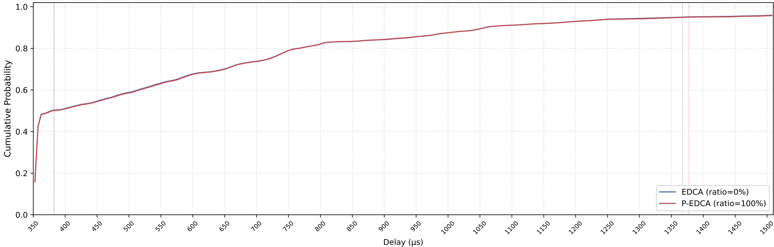
EDCA vs P-EDCA MAC Delay CDF — nSta=11, 1Mbps, avg of 10 runs
