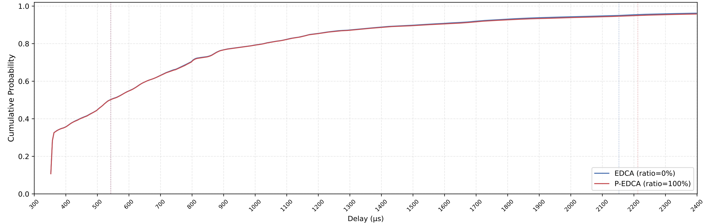
EDCA vs P-EDCA MAC Delay CDF — nSta=13, 1Mbps, avg of 10 runs
