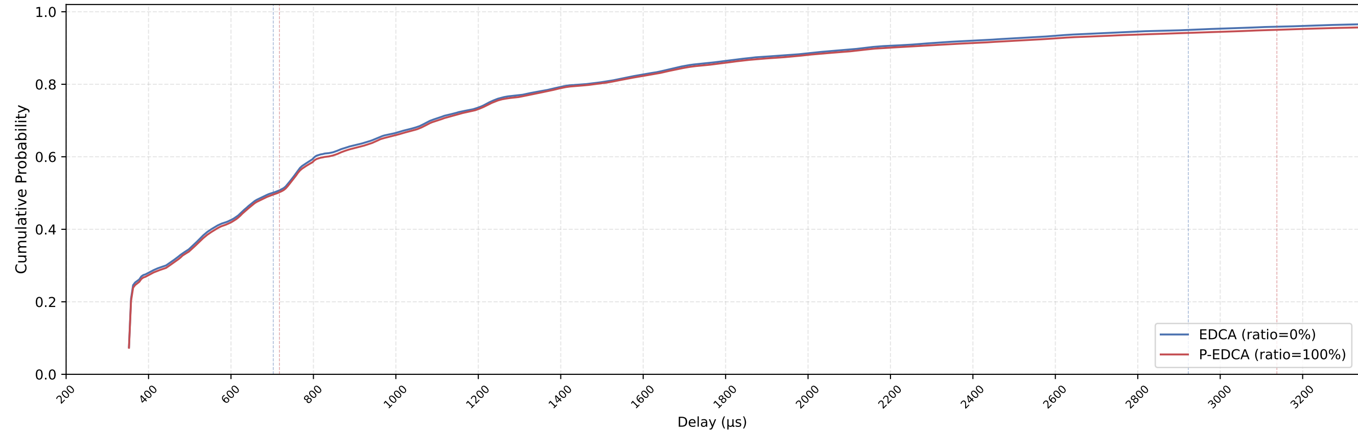
EDCA vs P-EDCA MAC Delay CDF — nSta=14, 1Mbps, avg of 10 runs
