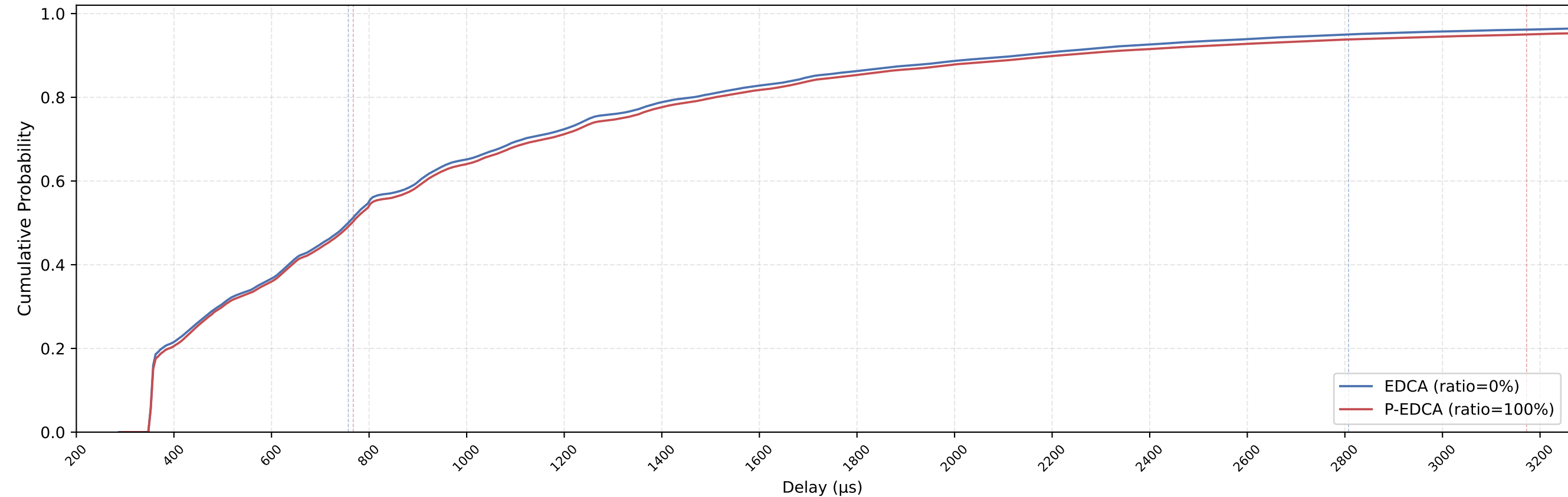
EDCA vs P-EDCA MAC Delay CDF — nSta=15, 1Mbps, avg of 10 runs
