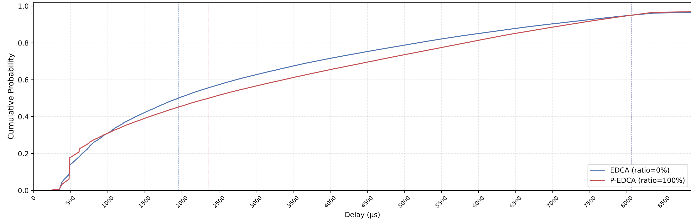
EDCA vs P-EDCA MAC Delay CDF — nSta=20, 1Mbps, avg of 10 runs
