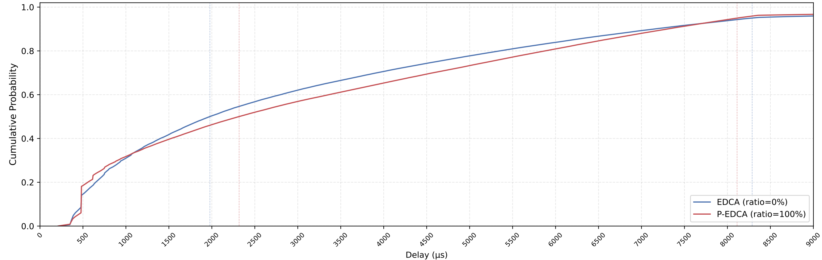
EDCA vs P-EDCA MAC Delay CDF — nSta=21, 1Mbps, avg of 10 runs
