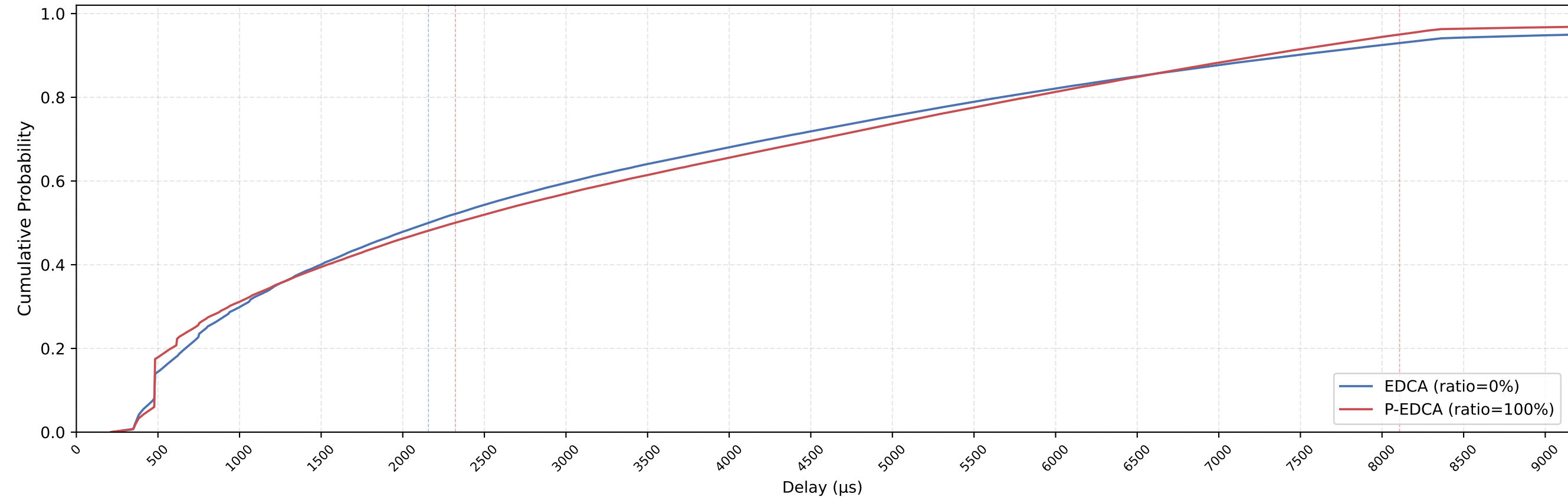
EDCA vs P-EDCA MAC Delay CDF — nSta=22, 1Mbps, avg of 10 runs
