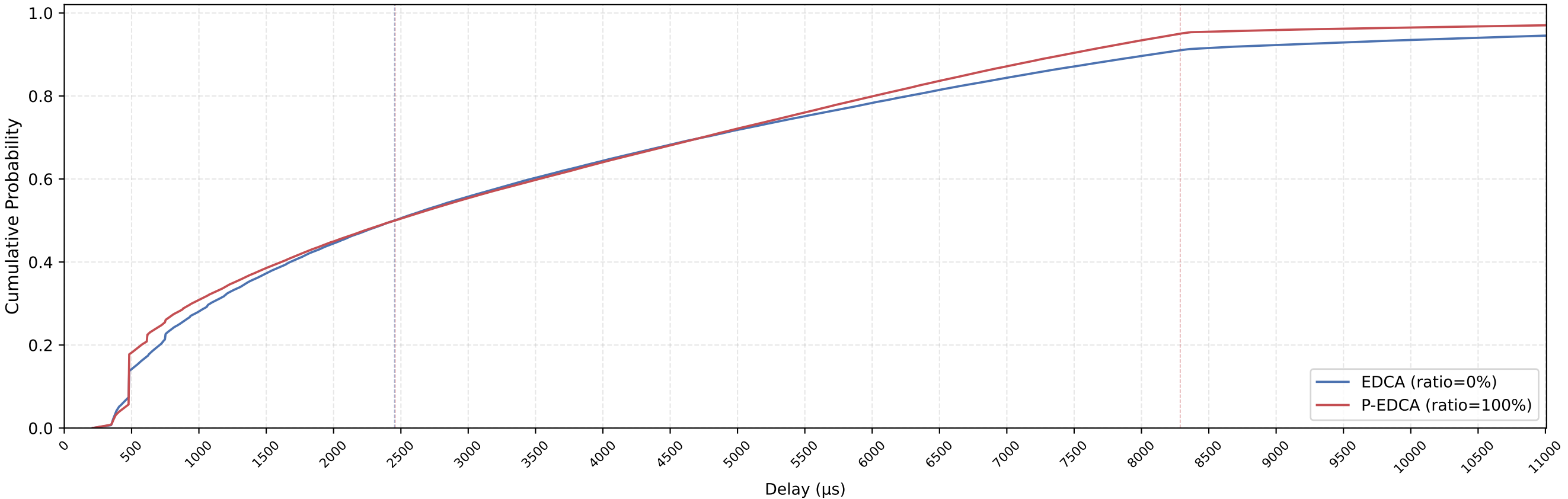
EDCA vs P-EDCA MAC Delay CDF — nSta=24, 1Mbps, avg of 10 runs
