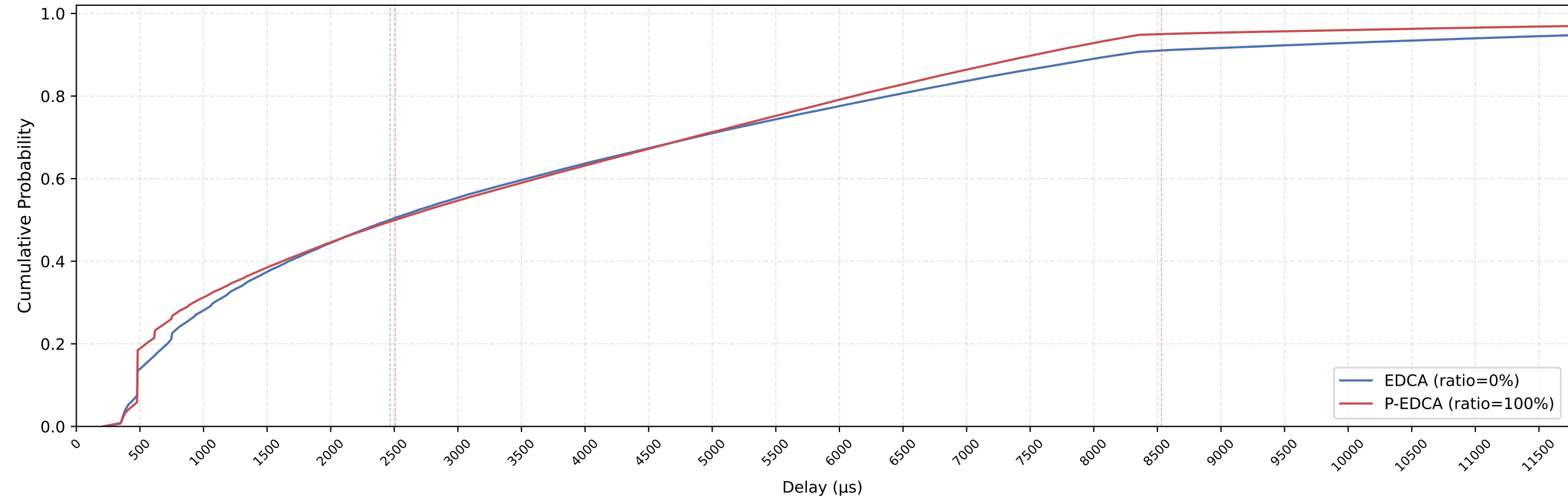
EDCA vs P-EDCA MAC Delay CDF — nSta=27, 1Mbps, avg of 10 runs
