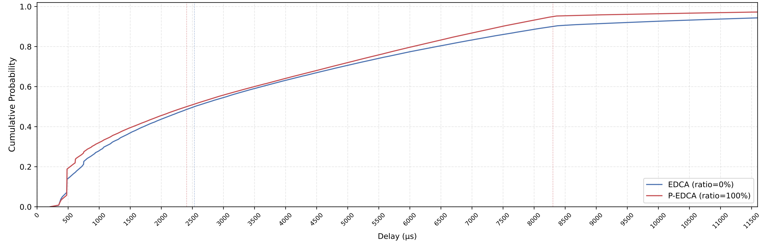
EDCA vs P-EDCA MAC Delay CDF — nSta=29, 1Mbps, avg of 10 runs
