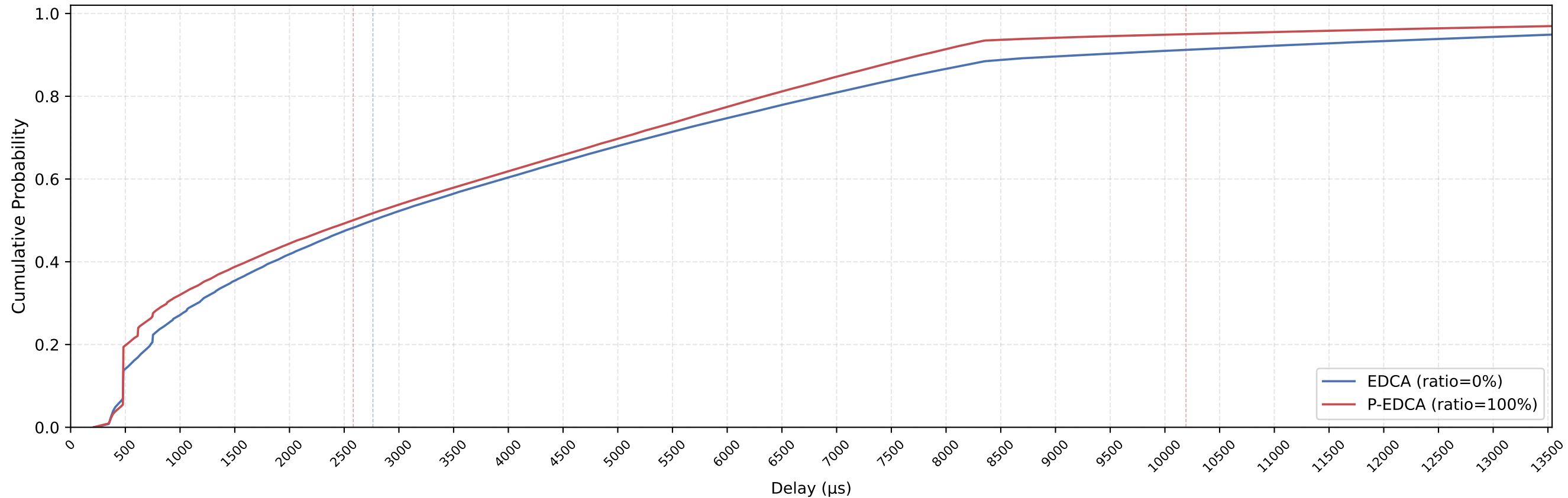
EDCA vs P-EDCA MAC Delay CDF — nSta=30, 1Mbps, avg of 10 runs
