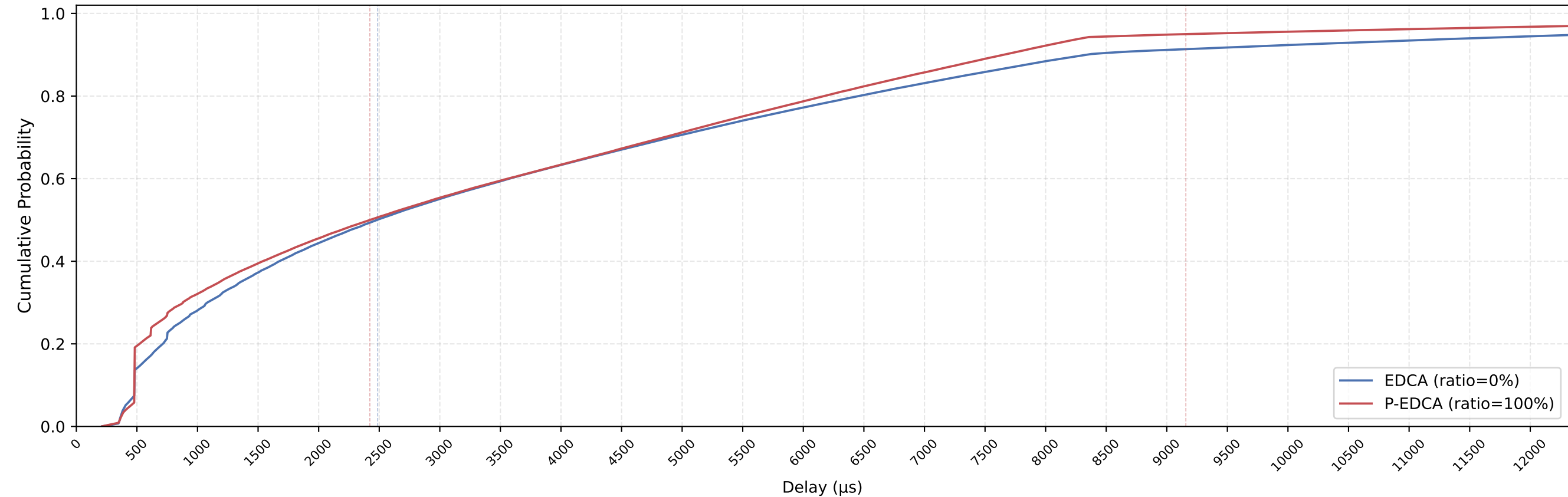
EDCA vs P-EDCA MAC Delay CDF — nSta=31, 1Mbps, avg of 10 runs
