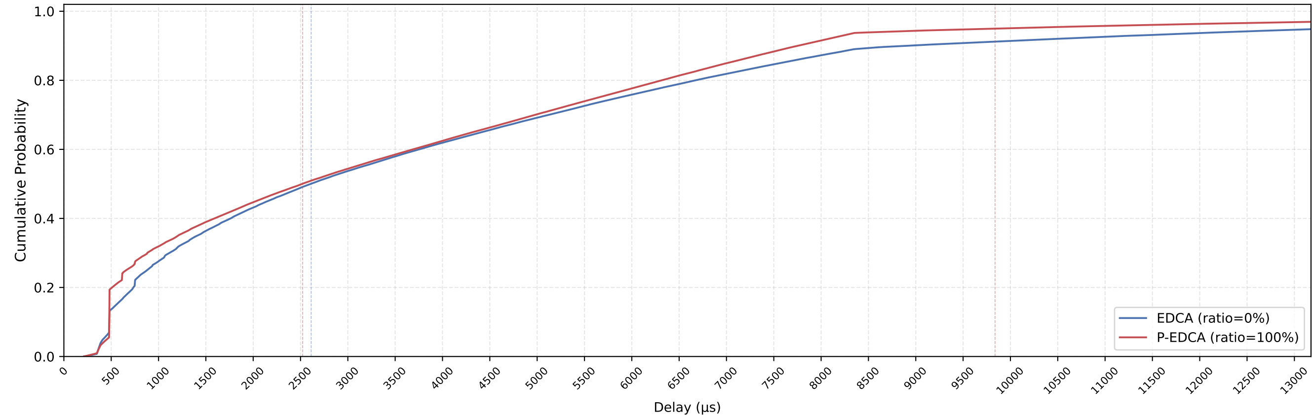
EDCA vs P-EDCA MAC Delay CDF — nSta=36, 1Mbps, avg of 10 runs
