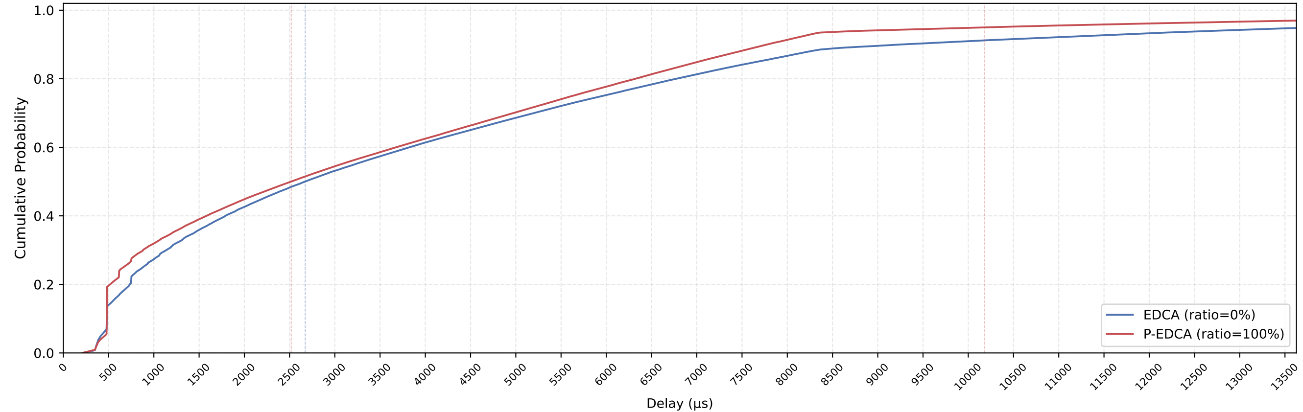
EDCA vs P-EDCA MAC Delay CDF — nSta=37, 1Mbps, avg of 10 runs
