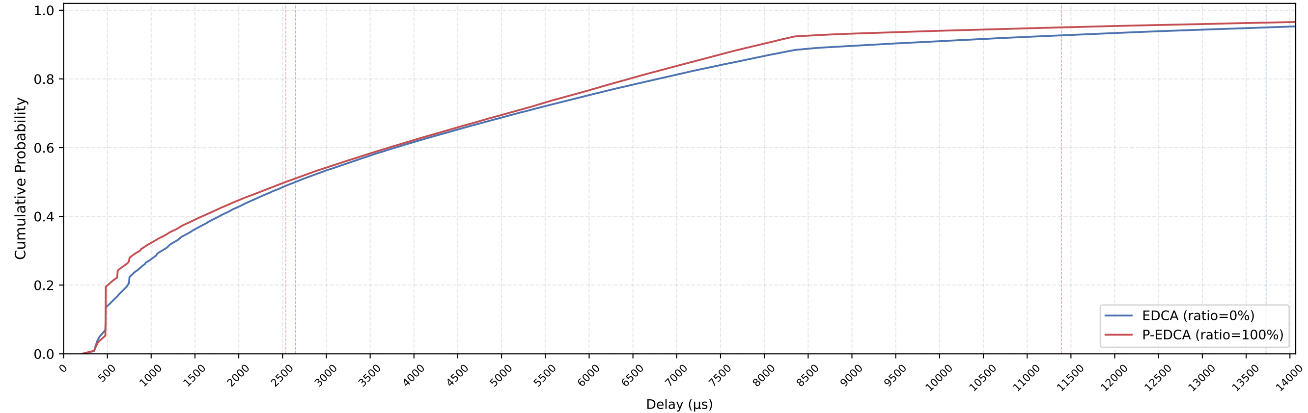
EDCA vs P-EDCA MAC Delay CDF — nSta=38, 1Mbps, avg of 10 runs
