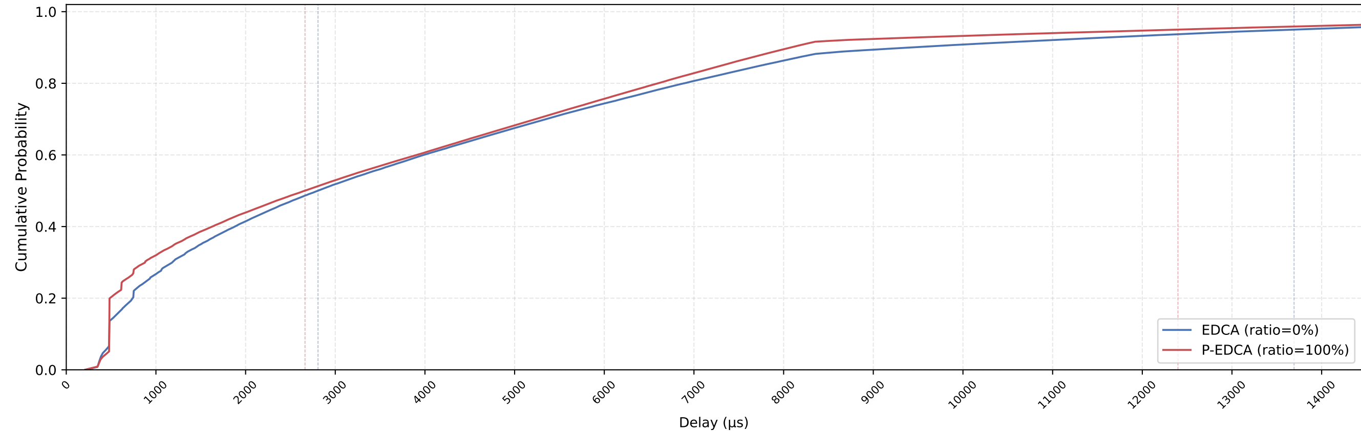
EDCA vs P-EDCA MAC Delay CDF — nSta=39, 1Mbps, avg of 10 runs
