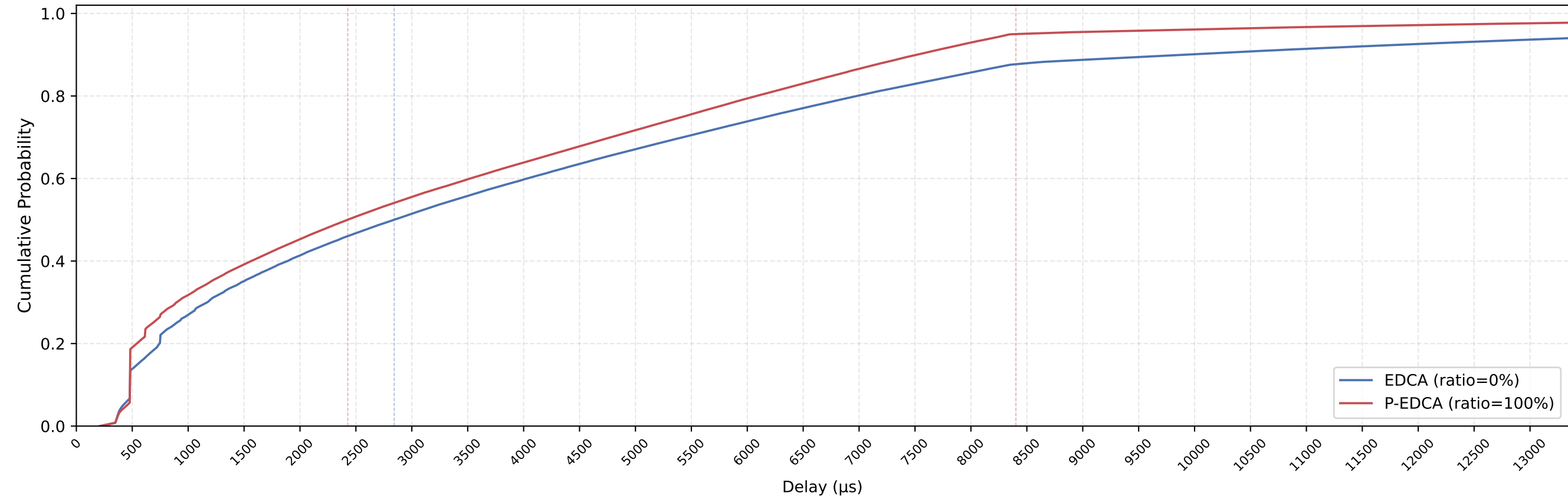
EDCA vs P-EDCA MAC Delay CDF — nSta=45, 1Mbps, avg of 10 runs
