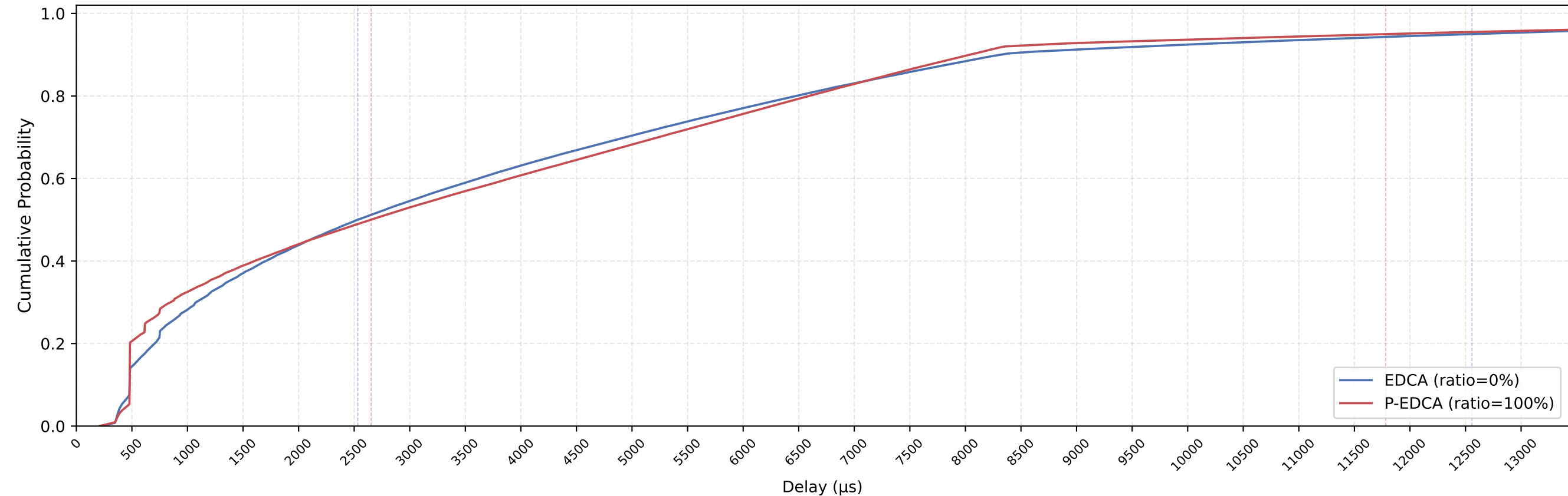
EDCA vs P-EDCA MAC Delay CDF — nSta=49, 1Mbps, avg of 10 runs
