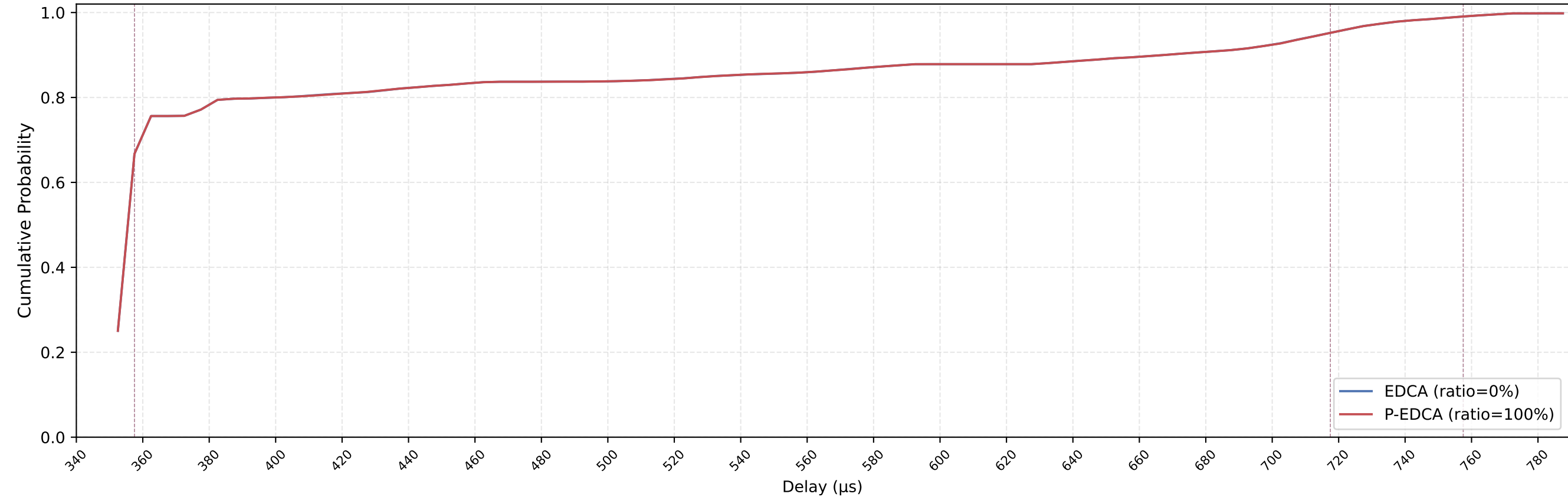
EDCA vs P-EDCA MAC Delay CDF — nSta=5, 1Mbps, avg of 10 runs
