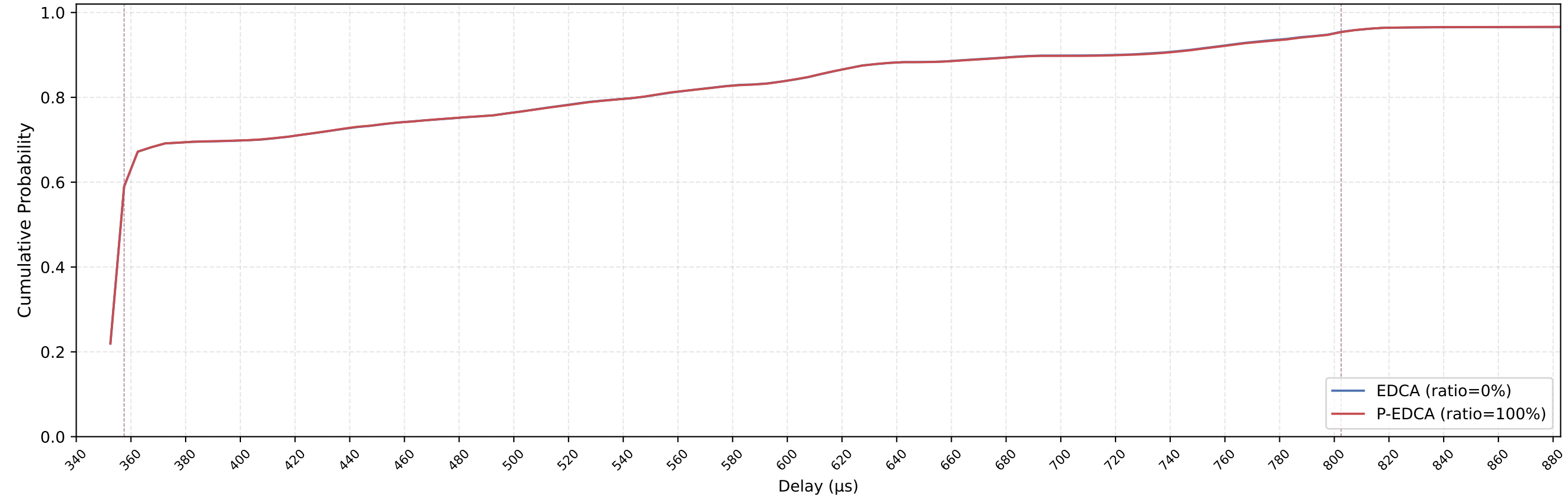
EDCA vs P-EDCA MAC Delay CDF — nSta=7, 1Mbps, avg of 10 runs
