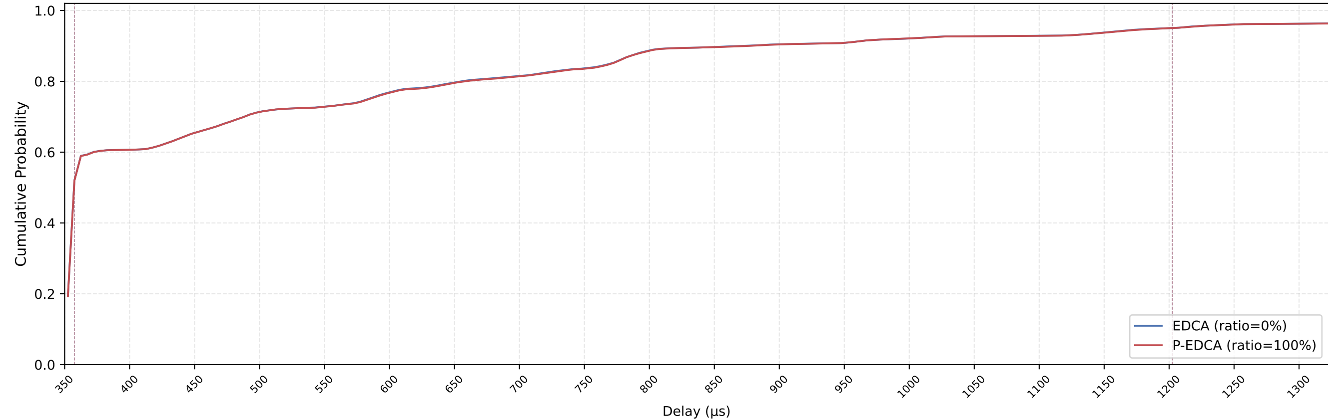
EDCA vs P-EDCA MAC Delay CDF — nSta=9, 1Mbps, avg of 10 runs
