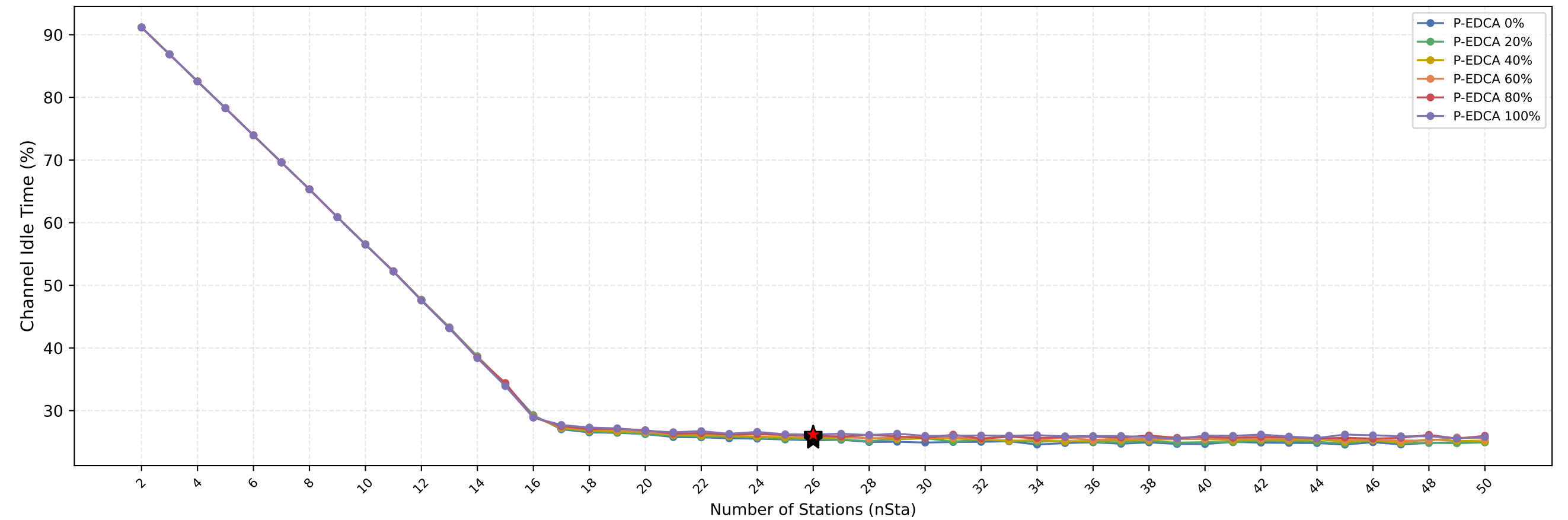
Channel Idle Time vs nSta — (Red Star = Current nSta=26)
