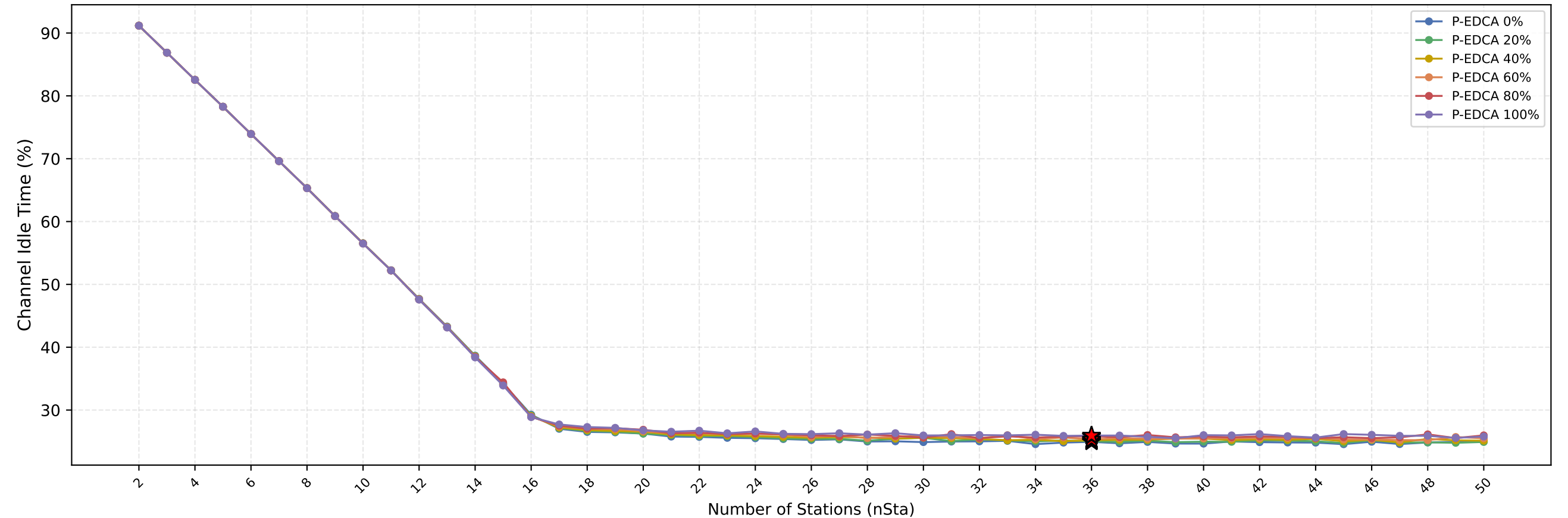
Channel Idle Time vs nSta — (Red Star = Current nSta=36)
