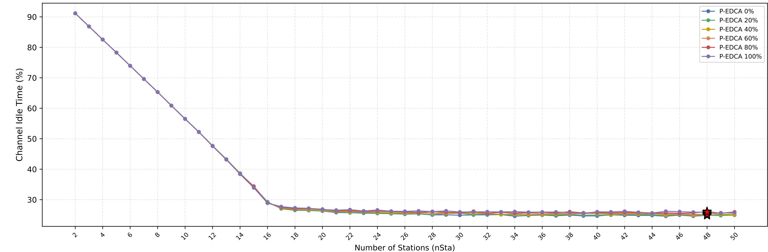
Channel Idle Time vs nSta — (Red Star = Current nSta=48)
