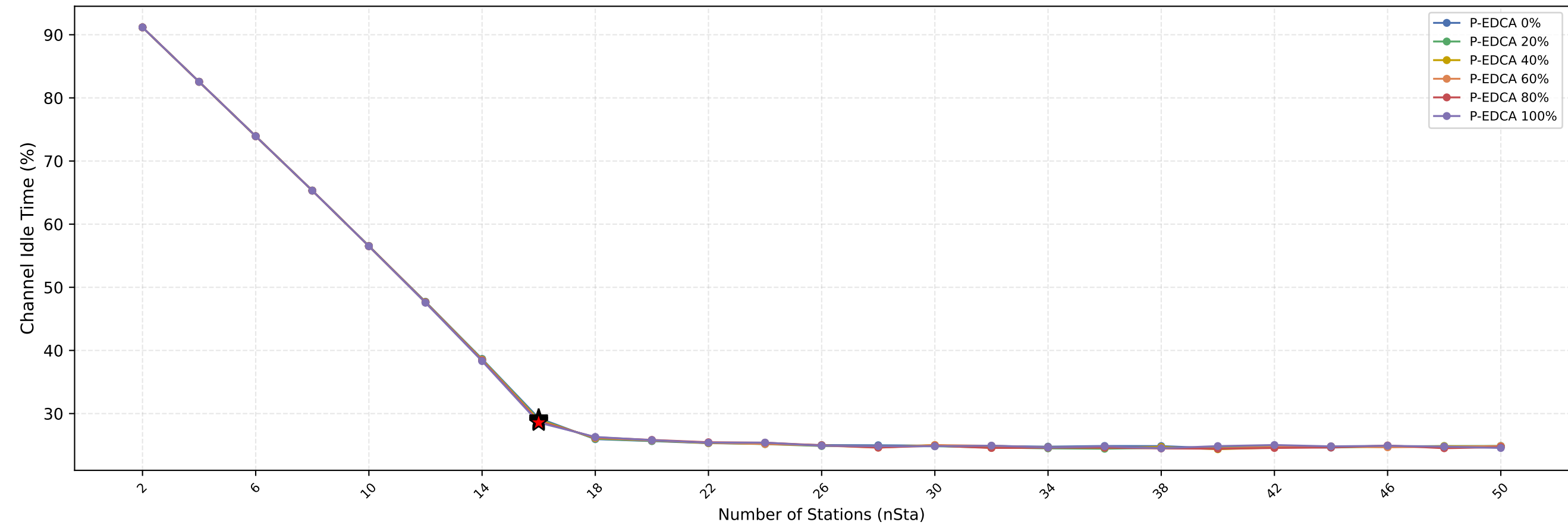
Channel Idle Time vs nSta — (Red Star = Current nSta=16)
