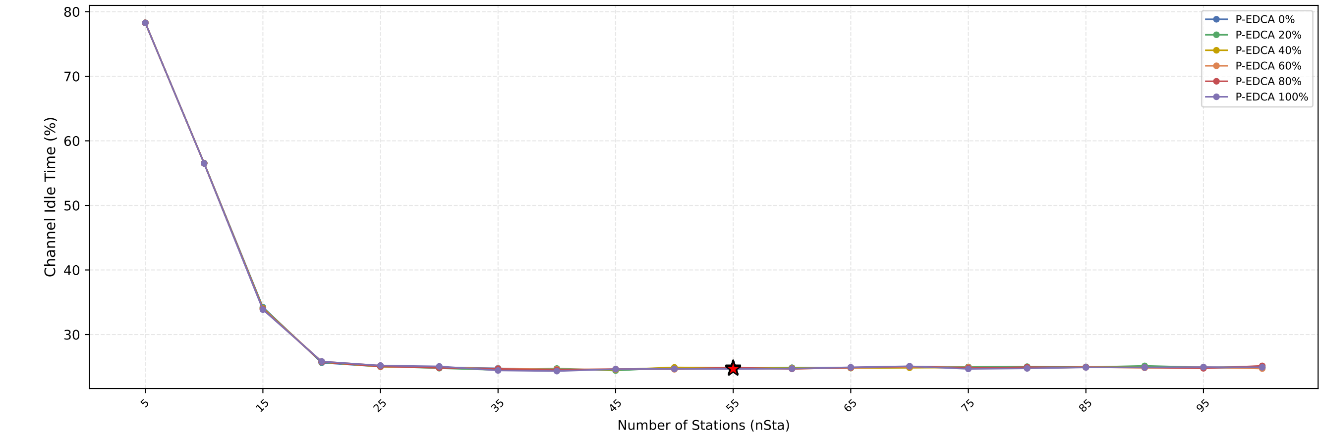
Channel Idle Time vs nSta — (Red Star = Current nSta=55)
