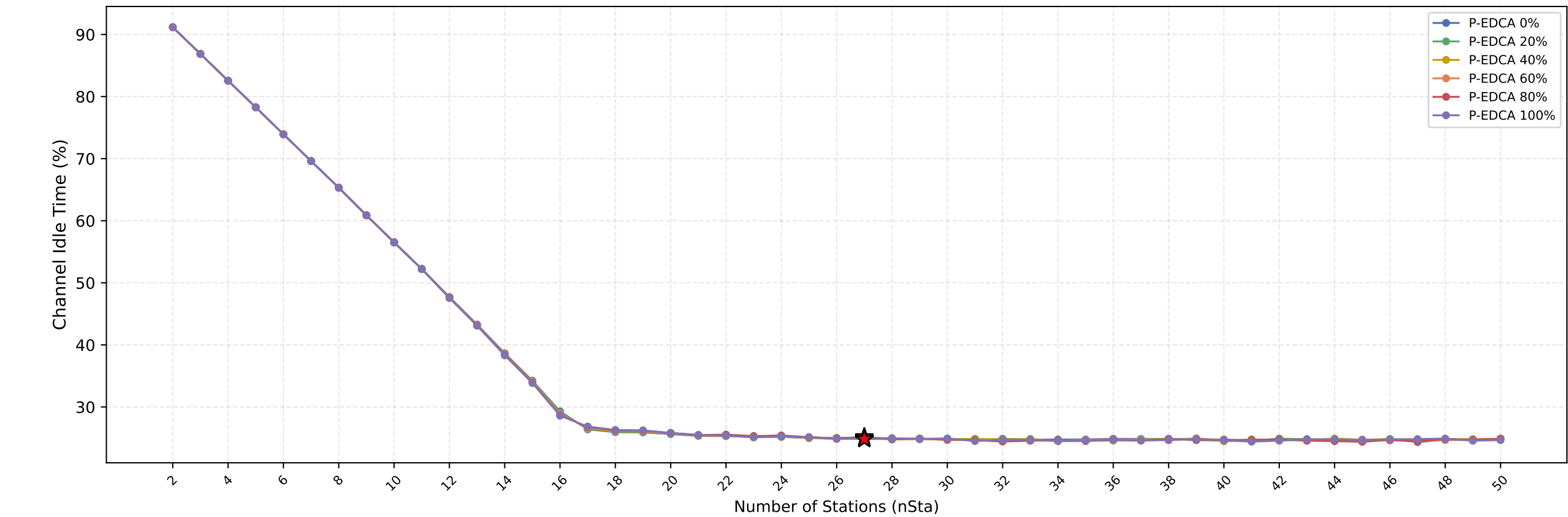
Channel Idle Time vs nSta — (Red Star = Current nSta=27)
