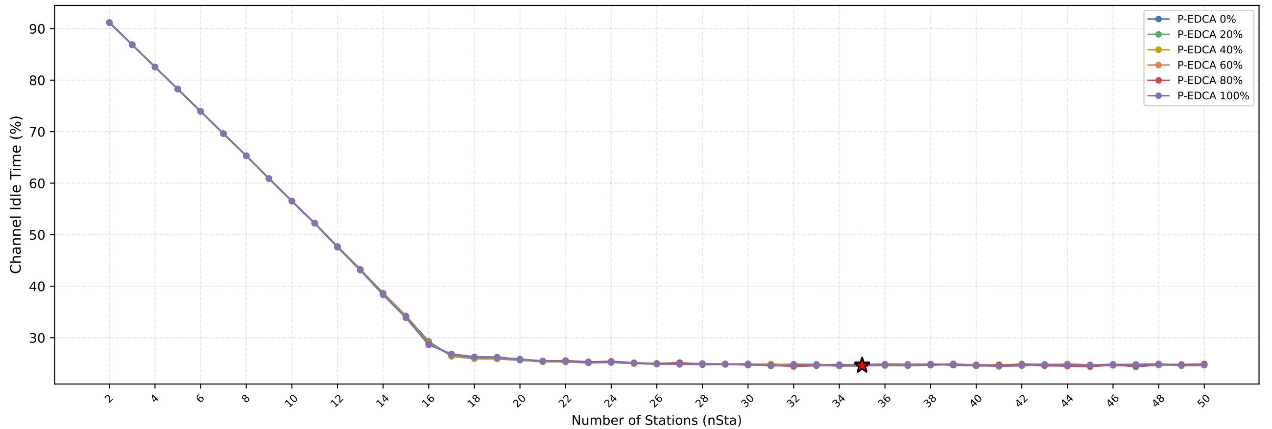
Channel Idle Time vs nSta — (Red Star = Current nSta=35)
