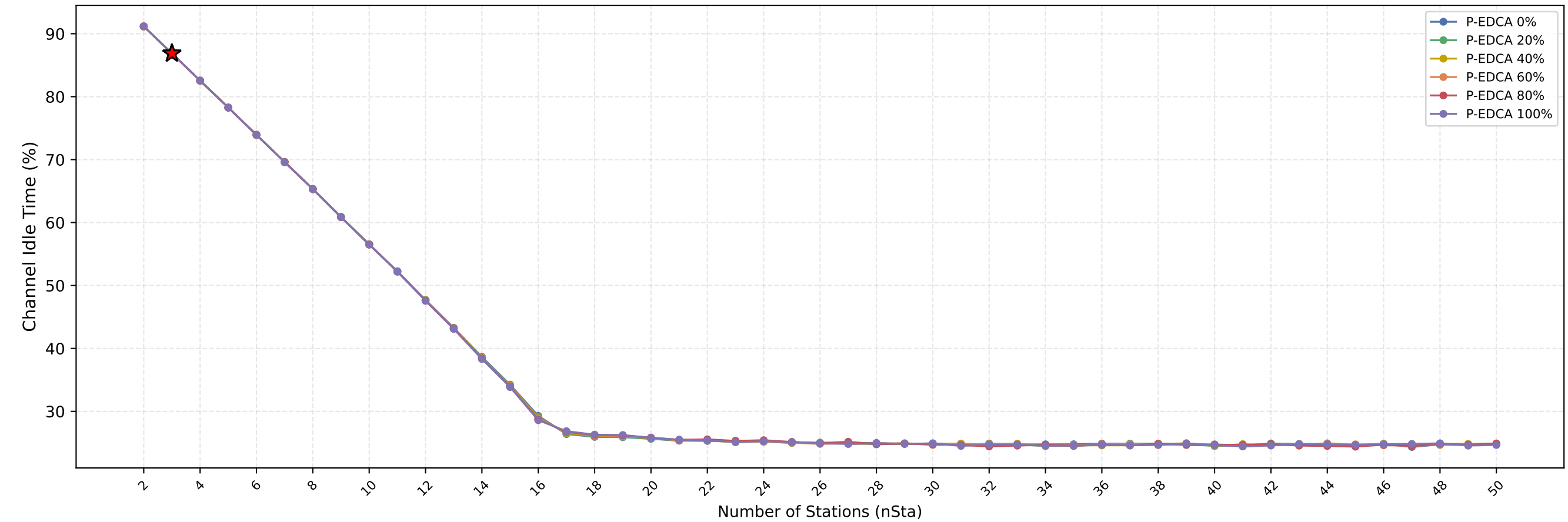
Channel Idle Time vs nSta — (Red Star = Current nSta=3)
