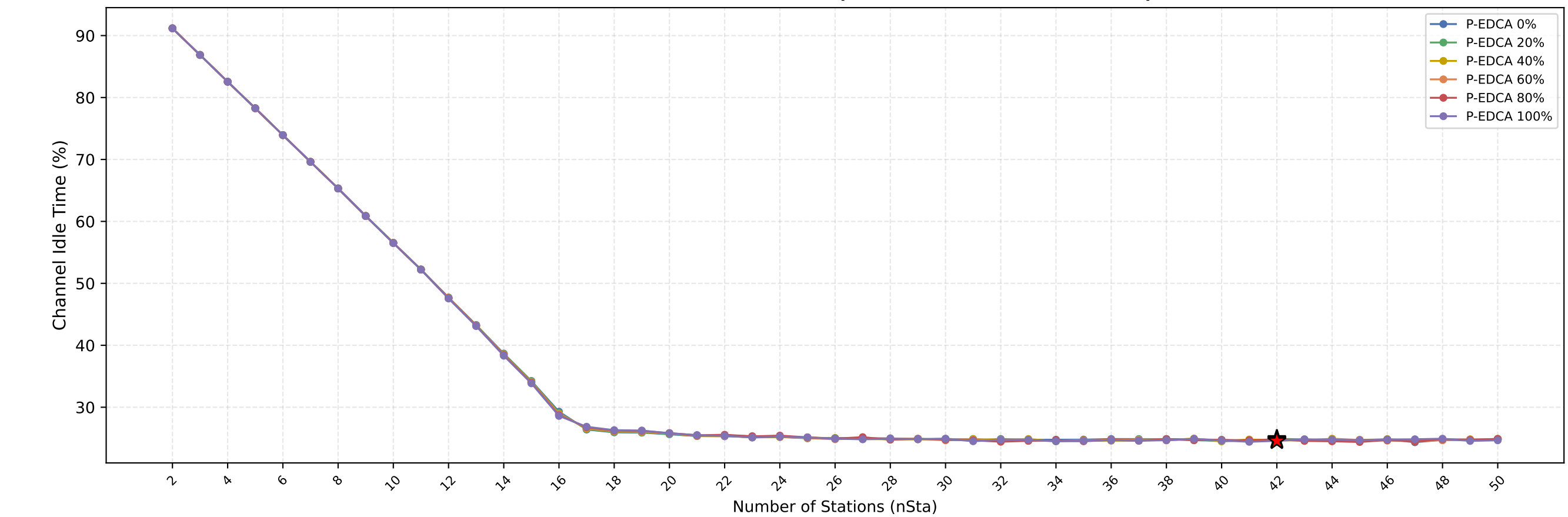
Channel Idle Time vs nSta — (Red Star = Current nSta=42)
