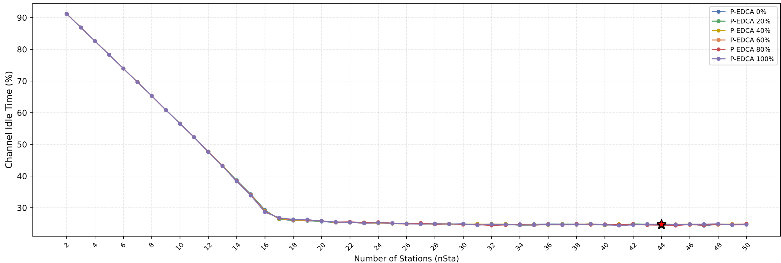
Channel Idle Time vs nSta — (Red Star = Current nSta=44)
