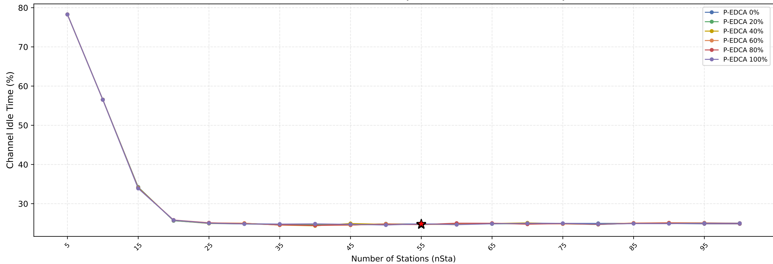
Channel Idle Time vs nSta — (Red Star = Current nSta=55)
