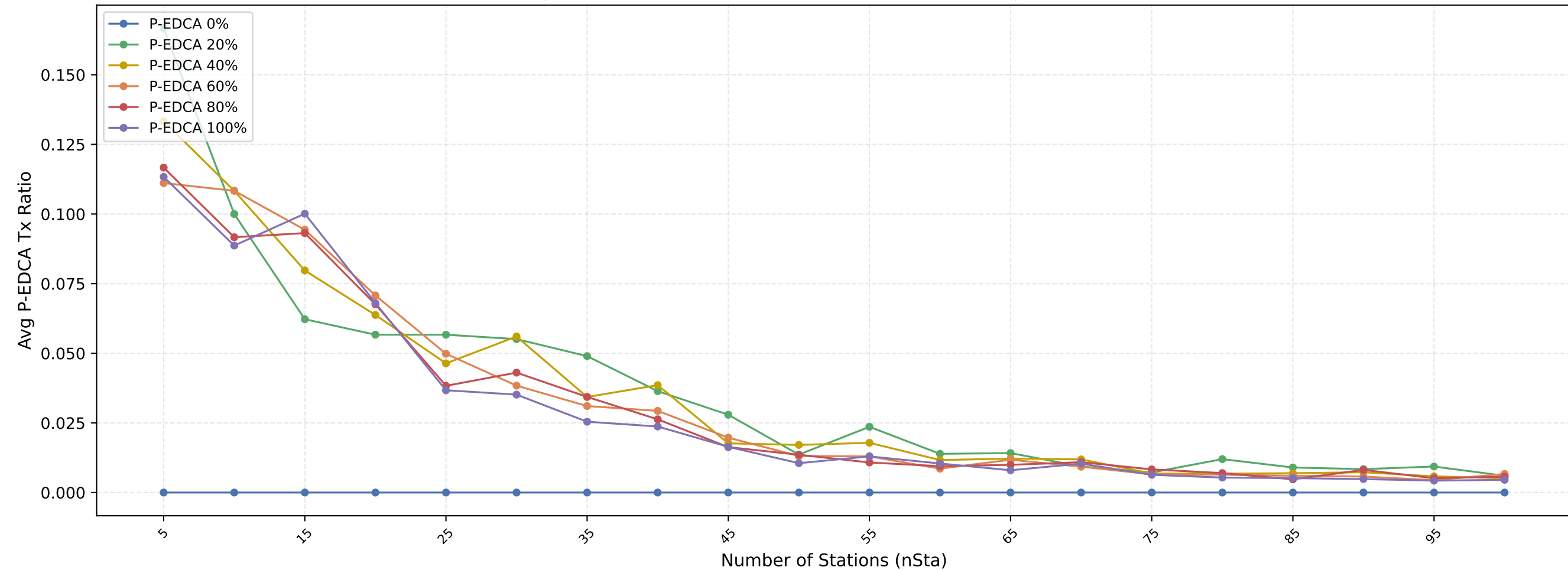
Avg P-EDCA Tx Ratio vs nSta — 1Mbps (avg of 10 runs)
