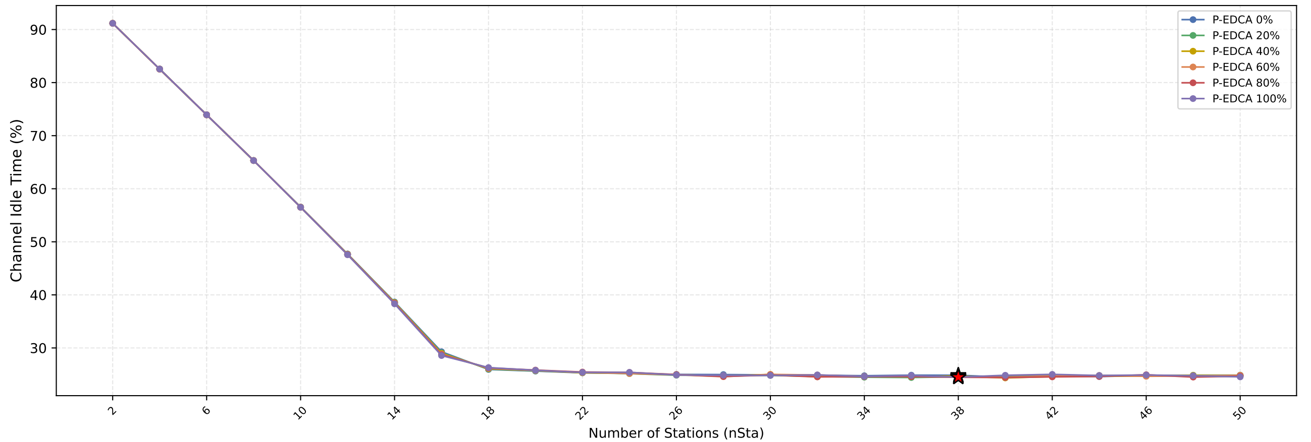
Channel Idle Time vs nSta — (Red Star = Current nSta=38)
