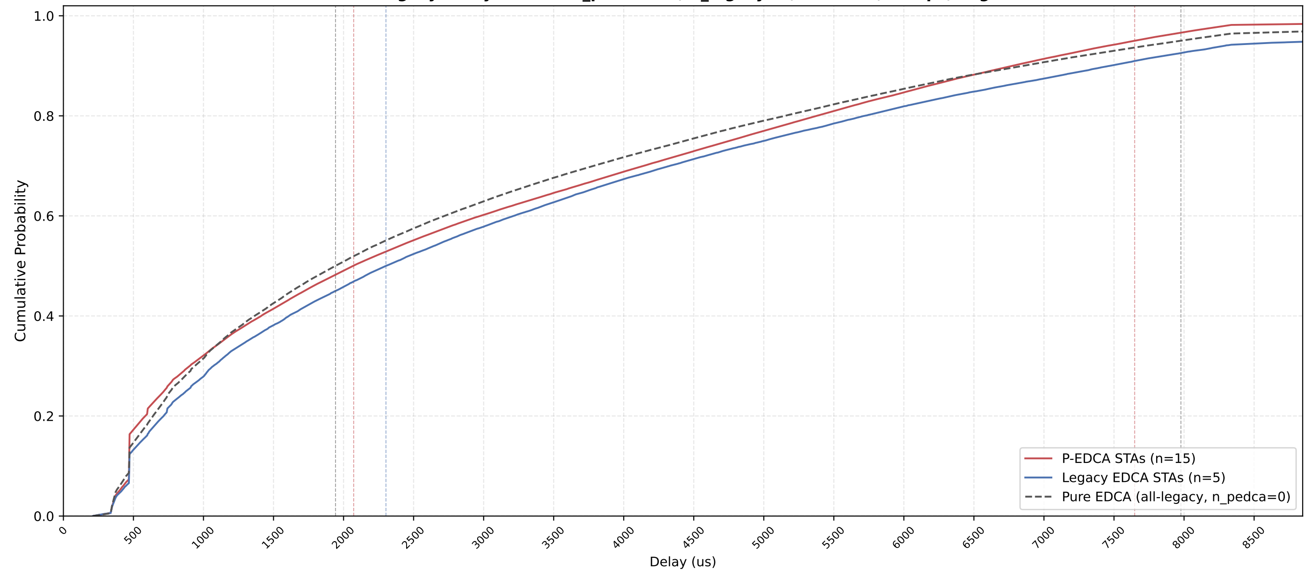
P-EDCA vs Legacy Delay CDF — n_pedca=15, n_legacy=5, nSta=20, 1Mbps, avg of 10 runs
