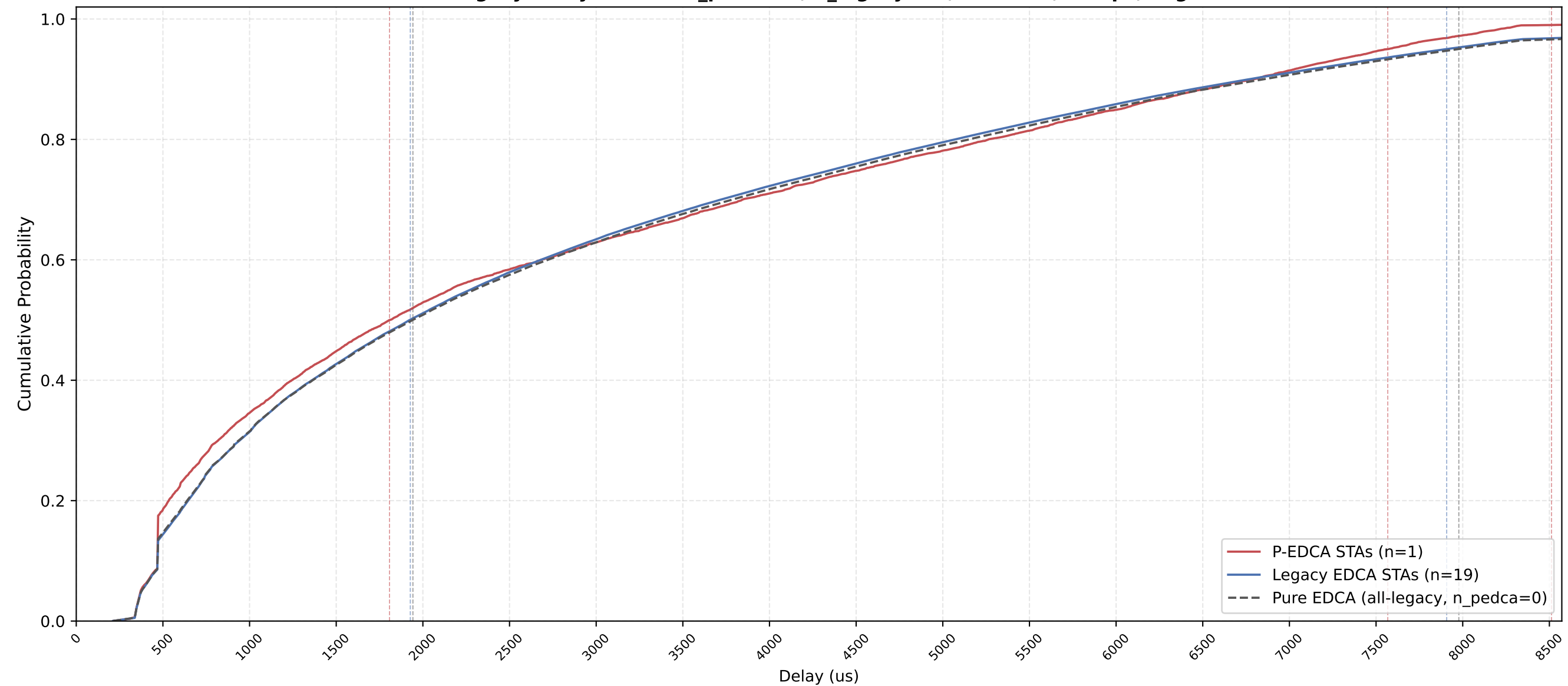
P-EDCA vs Legacy Delay CDF — n_pedca=1, n_legacy=19, nSta=20, 1Mbps, avg of 10 runs
