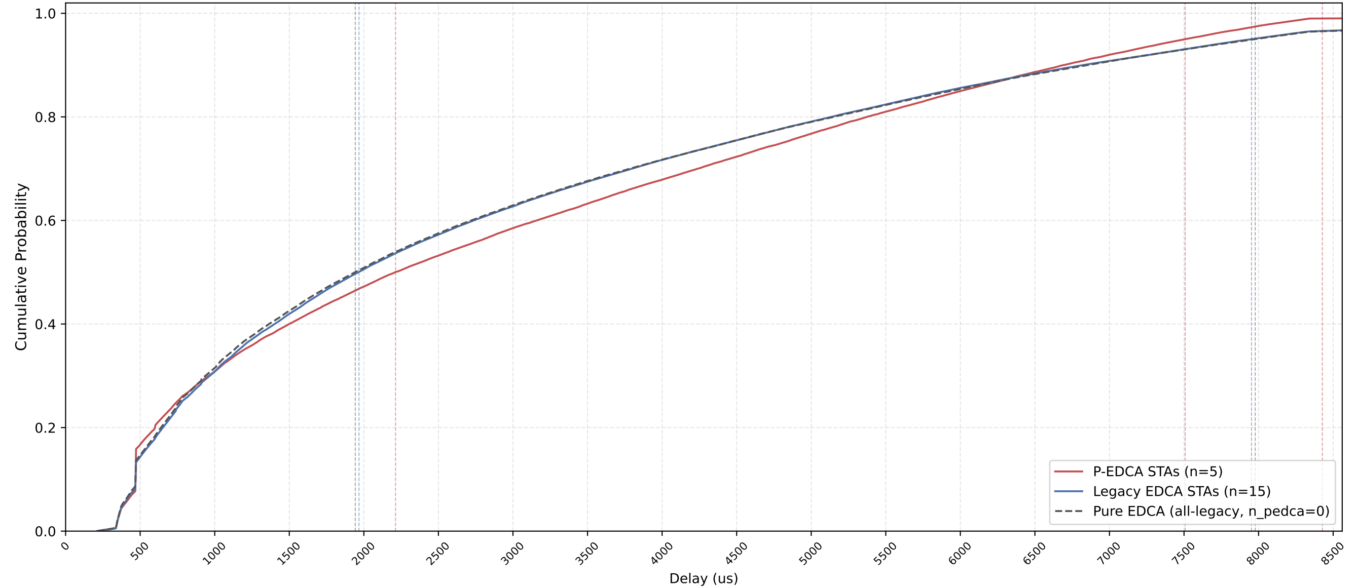
P-EDCA vs Legacy Delay CDF — n_pedca=5, n_legacy=15, nSta=20, 1Mbps, avg of 10 runs
