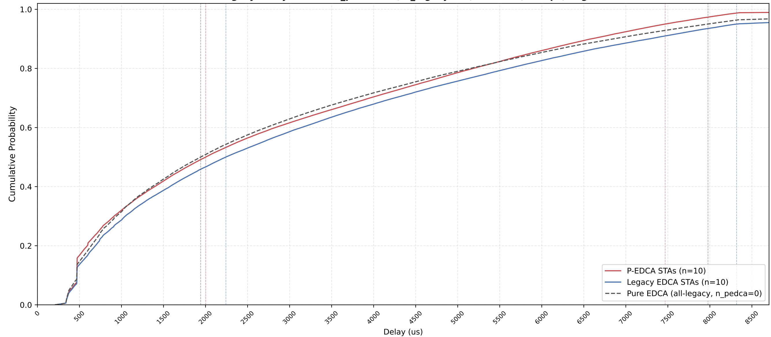
P-EDCA vs Legacy Delay CDF — n_pedca=10, n_legacy=10, nSta=20, 1Mbps, avg of 10 runs
