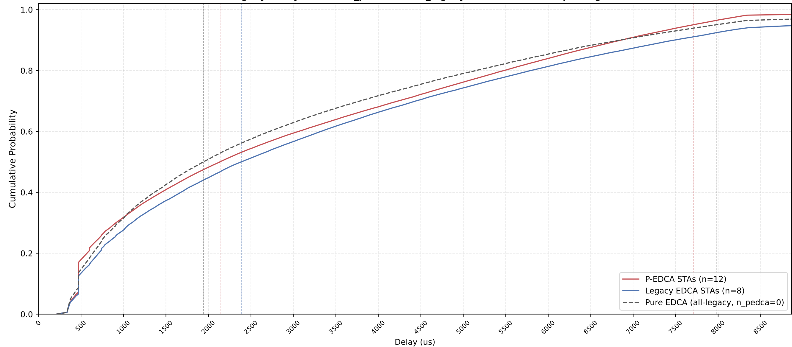
P-EDCA vs Legacy Delay CDF — n_pedca=12, n_legacy=8, nSta=20, 1Mbps, avg of 10 runs
