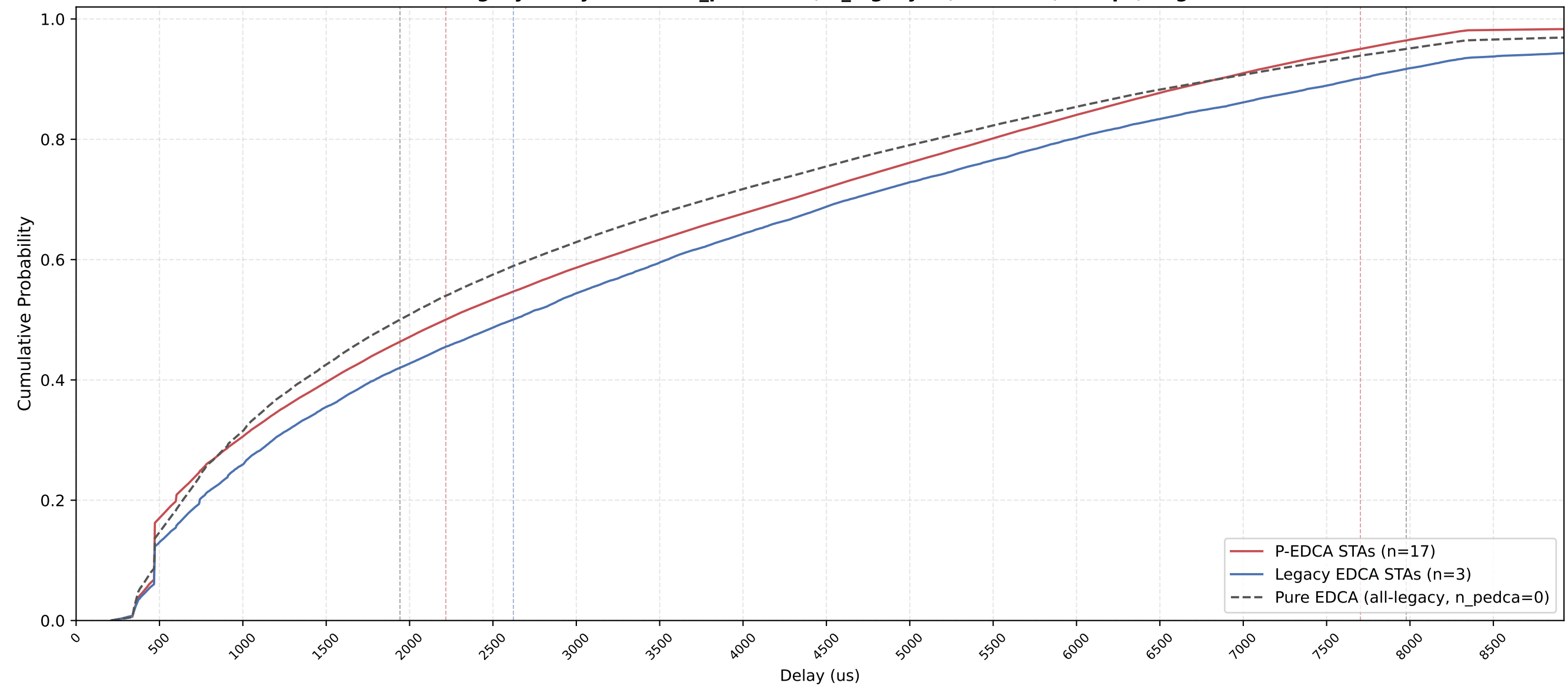
P-EDCA vs Legacy Delay CDF — n_pedca=17, n_legacy=3, nSta=20, 1Mbps, avg of 10 runs
