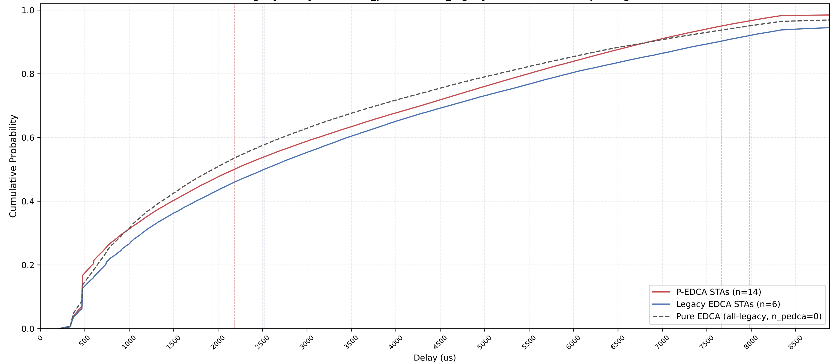
P-EDCA vs Legacy Delay CDF — n_pedca=14, n_legacy=6, nSta=20, 1Mbps, avg of 10 runs
