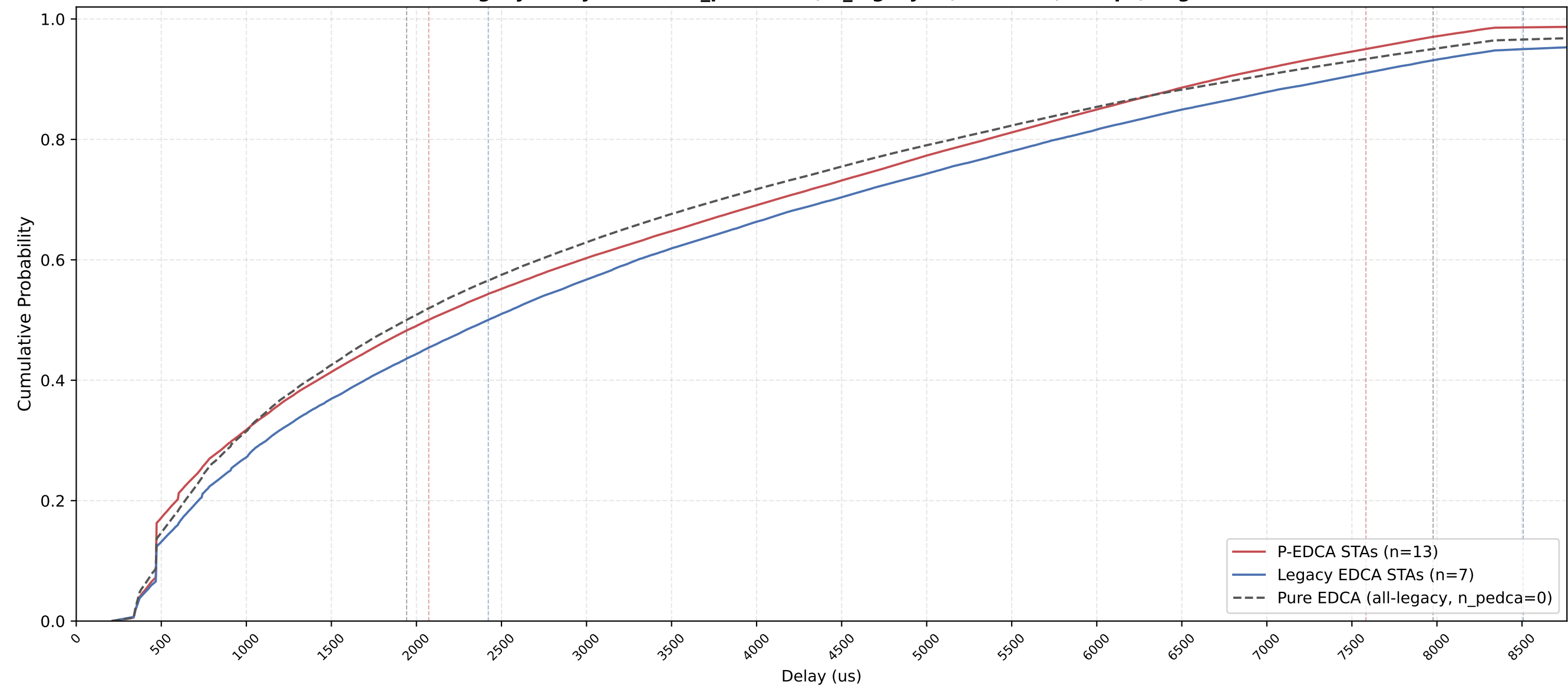
P-EDCA vs Legacy Delay CDF — n_pedca=13, n_legacy=7, nSta=20, 1Mbps, avg of 10 runs
