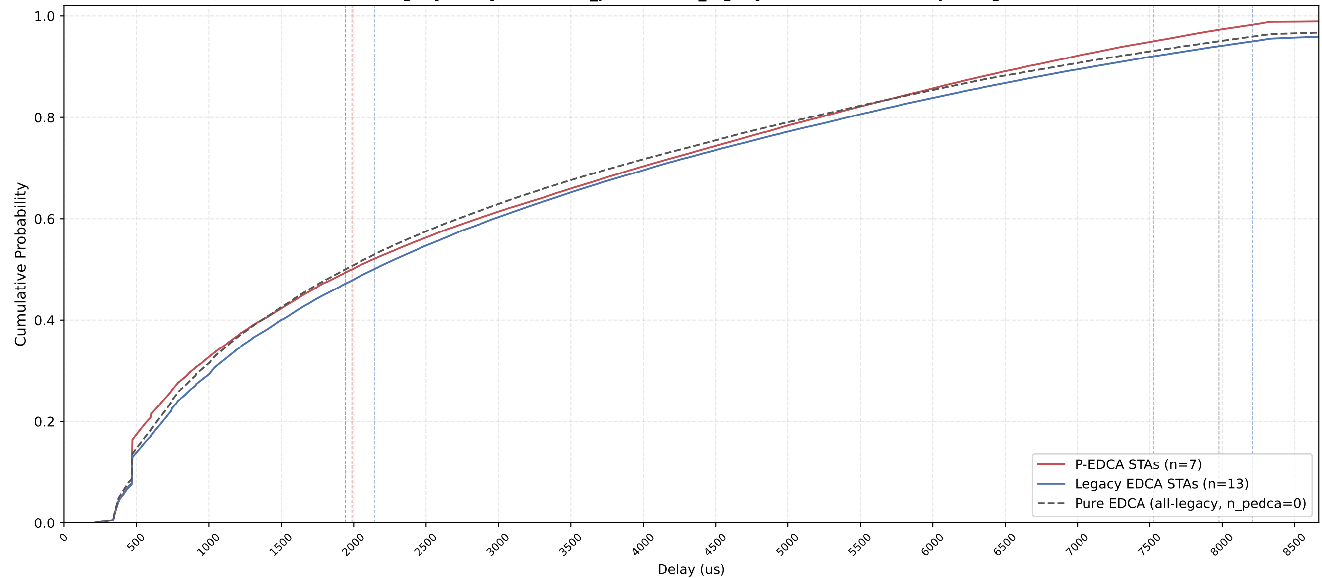
P-EDCA vs Legacy Delay CDF — n_pedca=7, n_legacy=13, nSta=20, 1Mbps, avg of 10 runs
