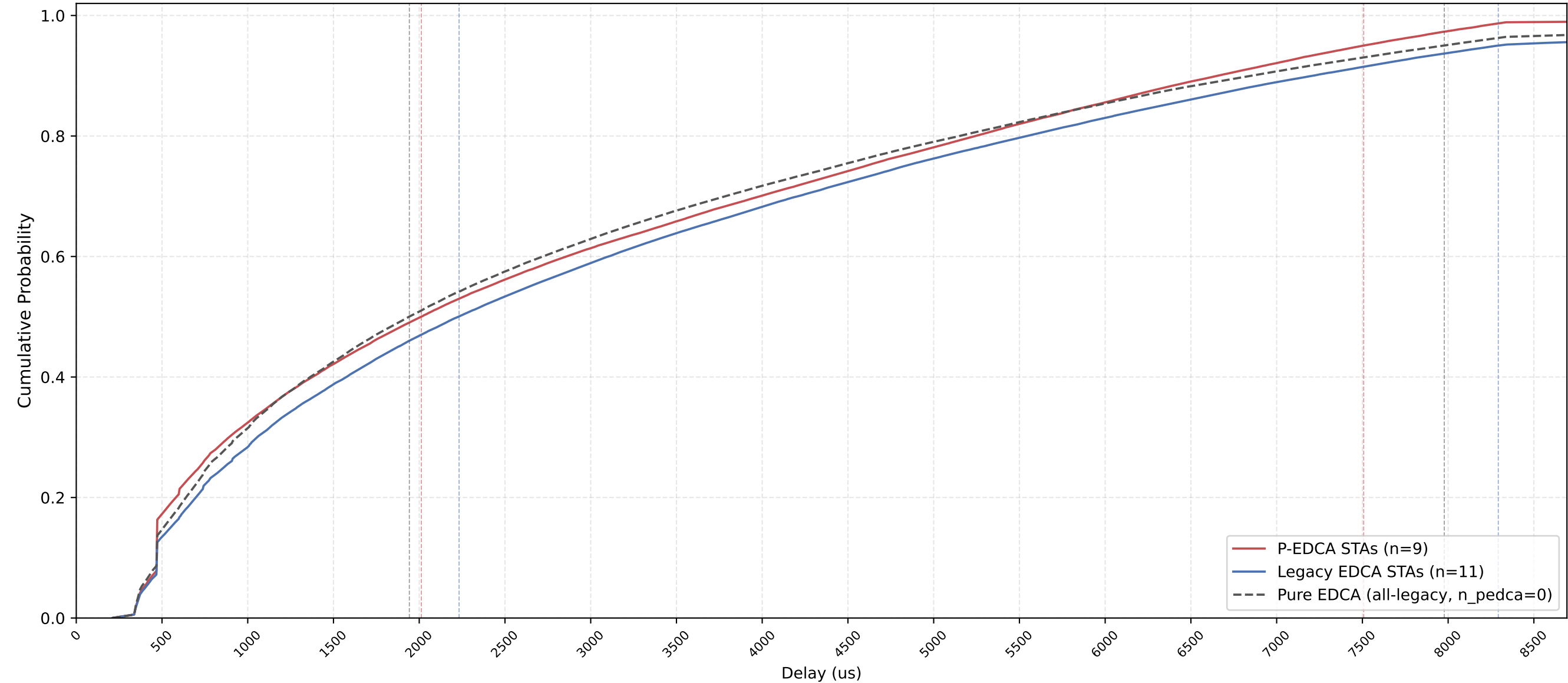
P-EDCA vs Legacy Delay CDF — n_pedca=9, n_legacy=11, nSta=20, 1Mbps, avg of 10 runs
