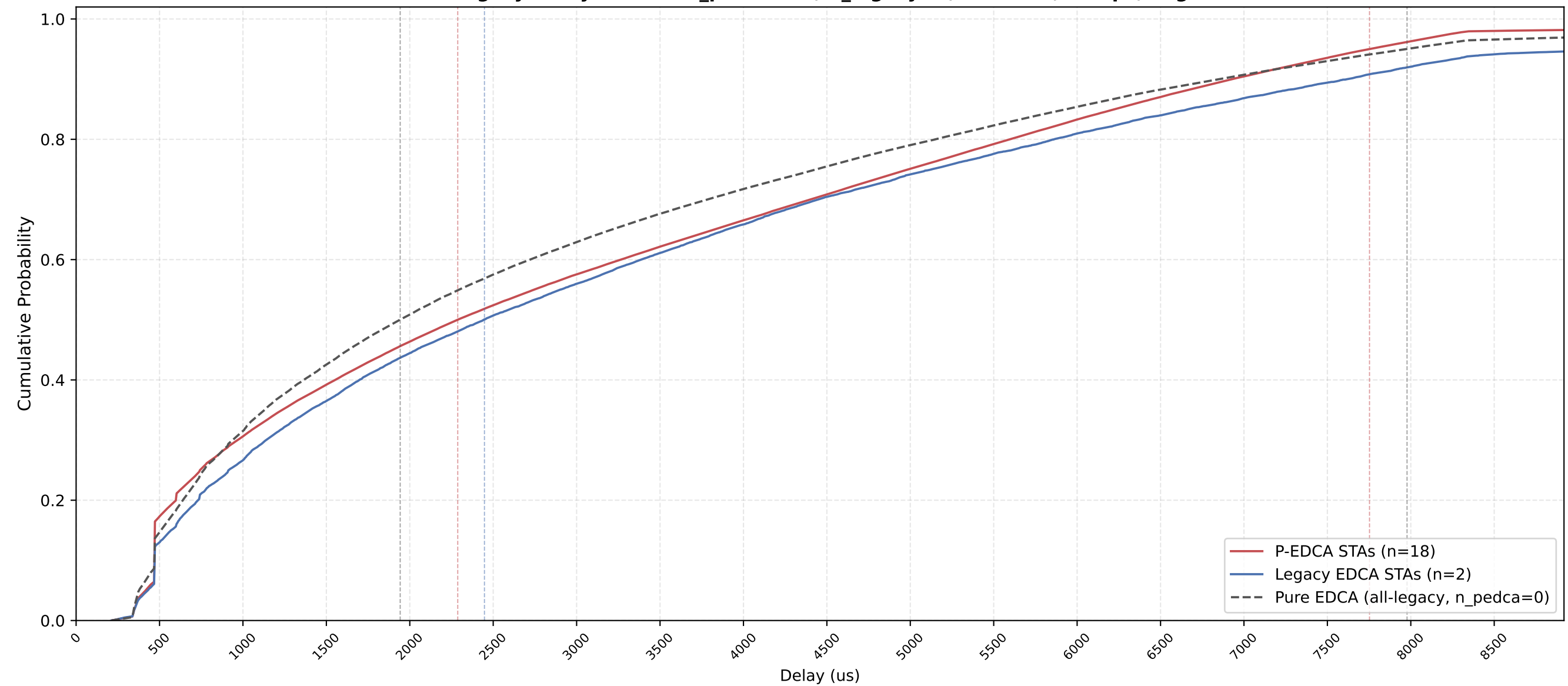
P-EDCA vs Legacy Delay CDF — n_pedca=18, n_legacy=2, nSta=20, 1Mbps, avg of 10 runs
