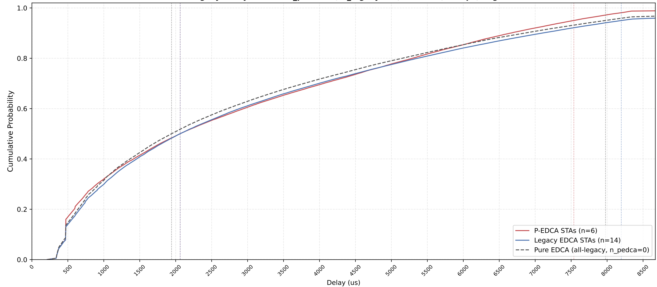
P-EDCA vs Legacy Delay CDF — n_pedca=6, n_legacy=14, nSta=20, 1Mbps, avg of 10 runs
