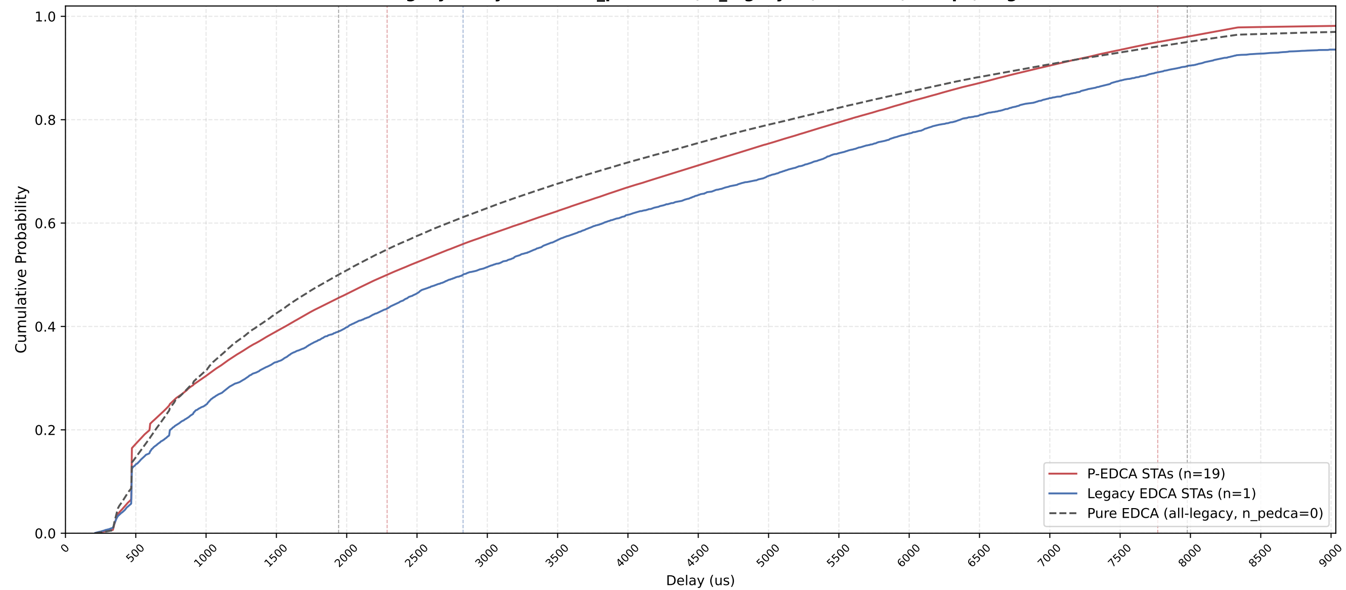
P-EDCA vs Legacy Delay CDF — n_pedca=19, n_legacy=1, nSta=20, 1Mbps, avg of 10 runs
