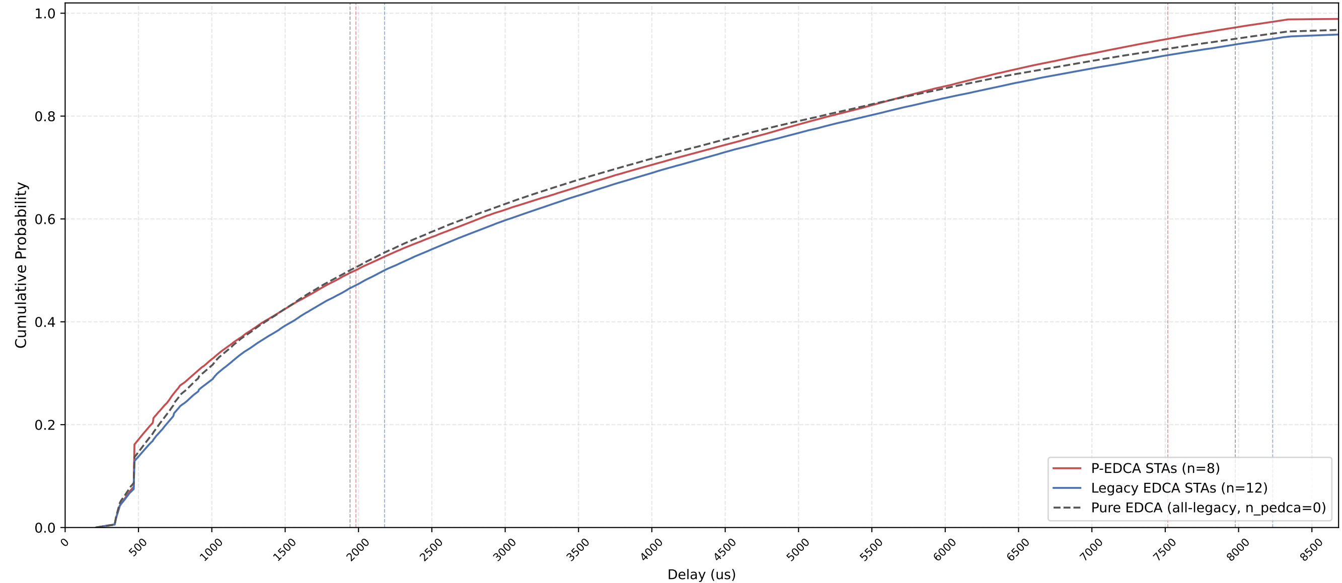
P-EDCA vs Legacy Delay CDF — n_pedca=8, n_legacy=12, nSta=20, 1Mbps, avg of 10 runs
