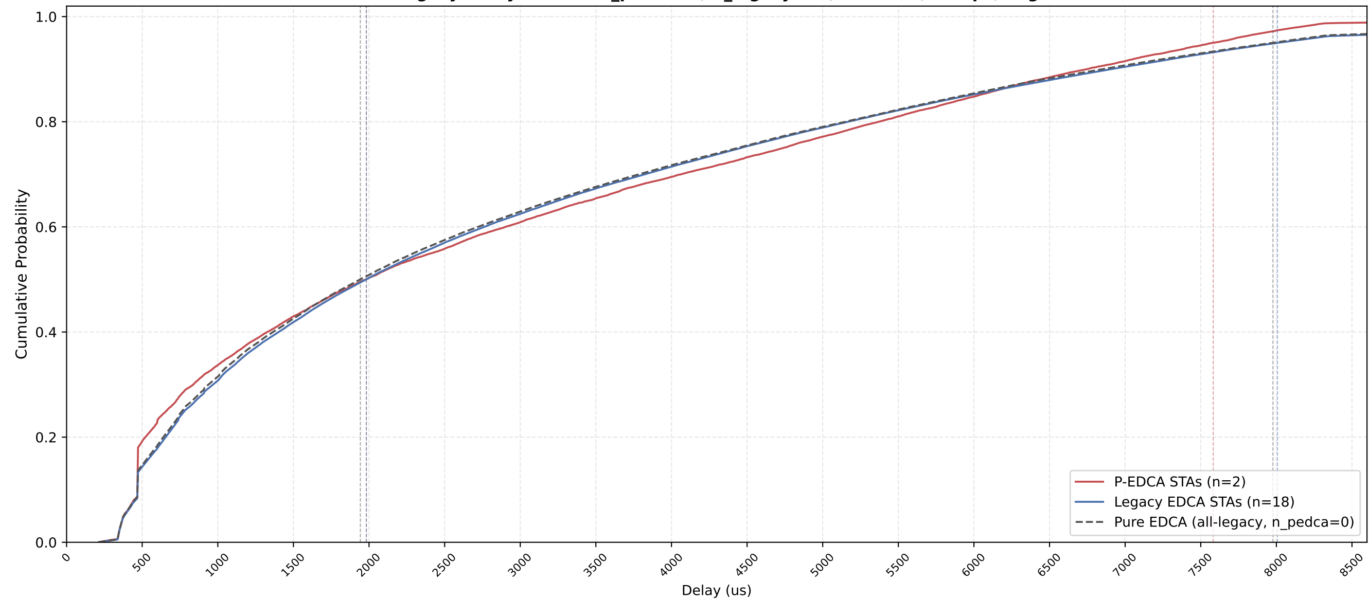
P-EDCA vs Legacy Delay CDF — n_pedca=2, n_legacy=18, nSta=20, 1Mbps, avg of 10 runs
