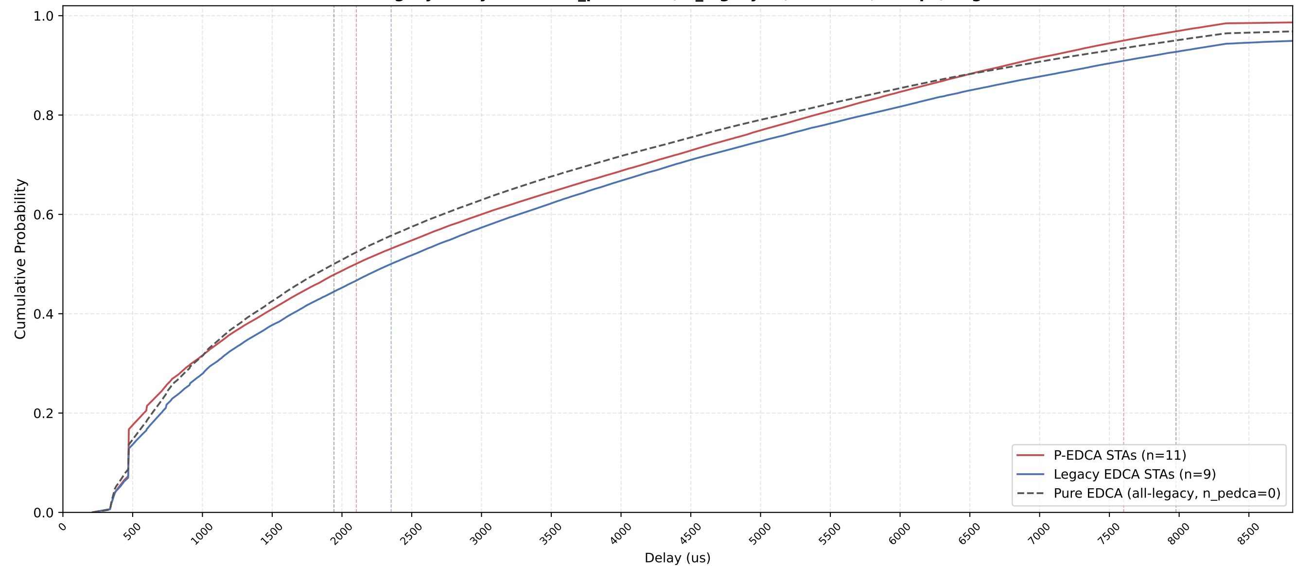
P-EDCA vs Legacy Delay CDF — n_pedca=11, n_legacy=9, nSta=20, 1Mbps, avg of 10 runs
