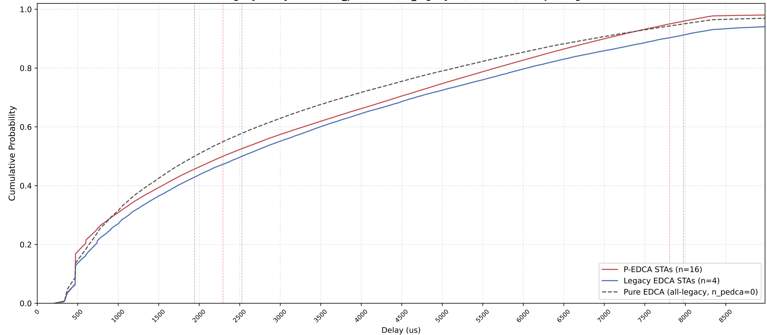
P-EDCA vs Legacy Delay CDF — n_pedca=16, n_legacy=4, nSta=20, 1Mbps, avg of 10 runs
