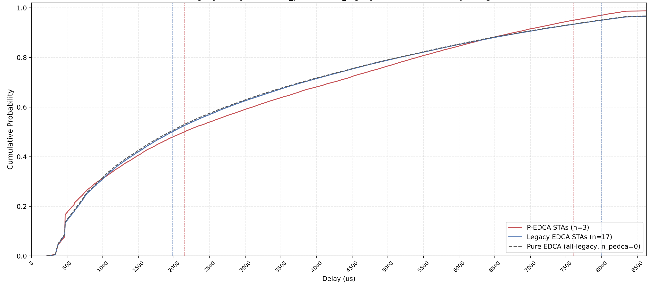
P-EDCA vs Legacy Delay CDF — n_pedca=3, n_legacy=17, nSta=20, 1Mbps, avg of 10 runs
