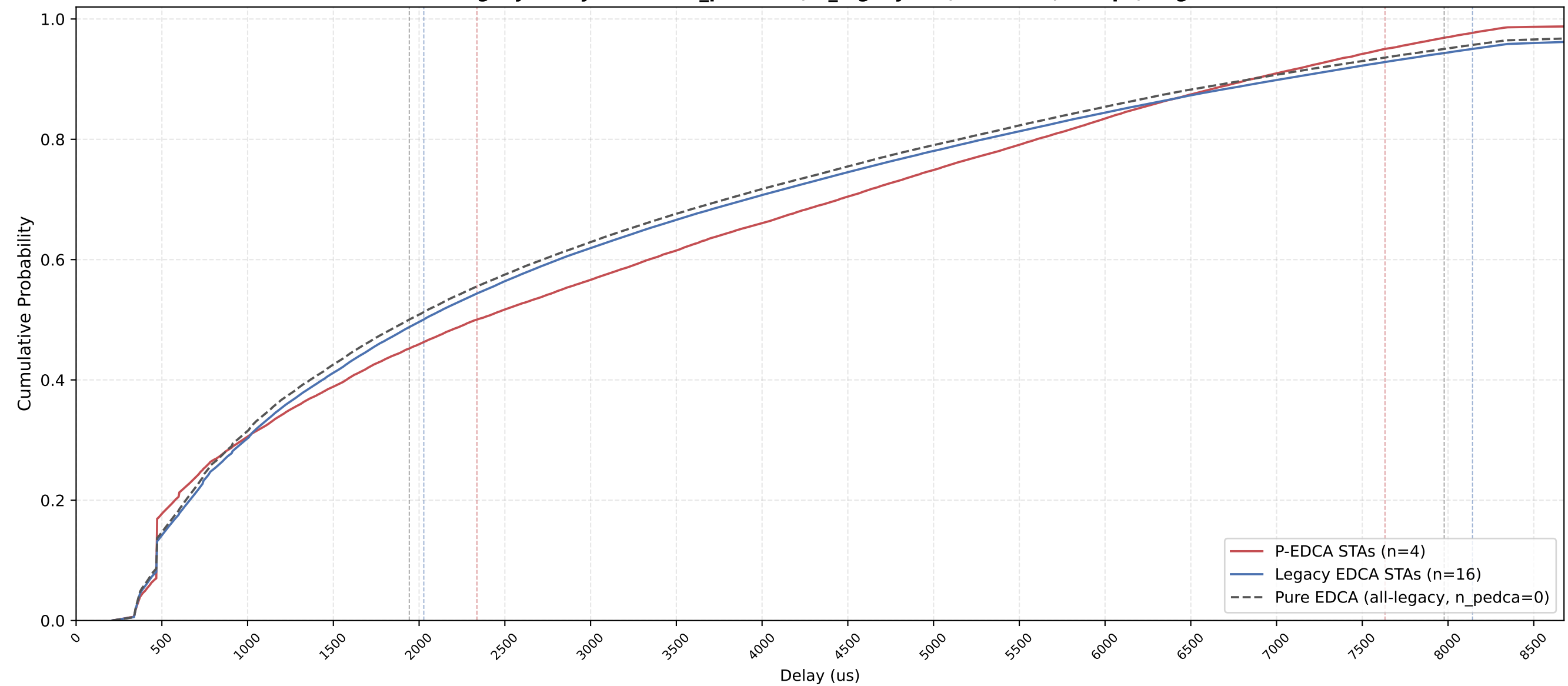
P-EDCA vs Legacy Delay CDF — n_pedca=4, n_legacy=16, nSta=20, 1Mbps, avg of 10 runs
