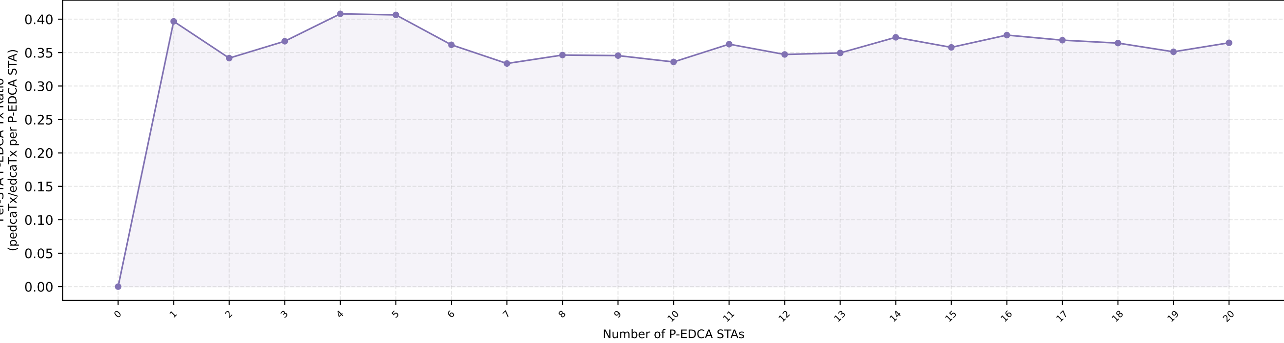
P-EDCA Success Rate: pedcaTx / pedcaAttempt — nSta=20, 1Mbps (avg of 10 runs)
